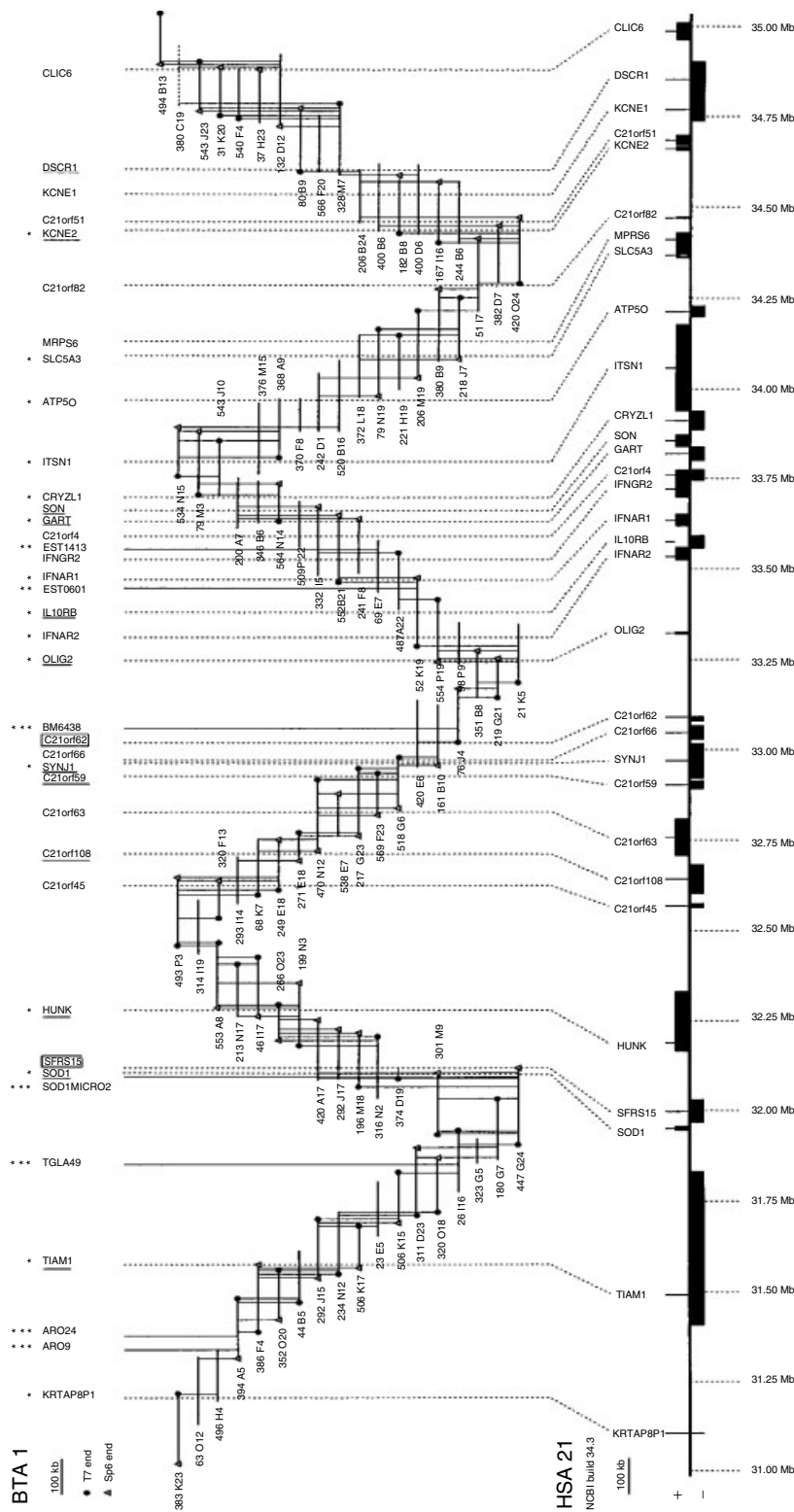
Figure 1. Physical map of the isolated bovine BAC contig on BTA 1q12. All mapped loci are indicated vertically at the top. Previously published BTA 1 mapping results are marked by one (genes), two (ESTs) or three (microsatellites) asterisks. Underlined gene markers were initially assigned by human cDNA hybridization probes. The two framed genes were localized on the contig in silico . RPCI-42 BAC clones are shown below the markers as continuous horizontal lines with their corresponding abbreviated clone names. A single chimeric BAC is shown by a dashed horizontal line. A minimal tiling path of 32 clones is indicated by thick lines. Bovine microsatellite, EST and STS markers are represented by vertical solid lines. Bovine markers that are associated to corresponding human genes are plotted by dotted vertical lines and linked to 31 genes on the 4 Mb sequence segment of HSA 21q22 (NCBI build 34.3) at the bottom. Comparative mapping of 31 gene-associated markers revealed a complete conservation of the gene order across the entire 4 Mb interval between Bos taurus and Homo sapiens
