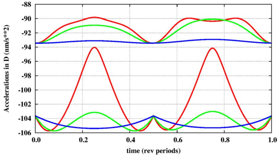
GPS Block IIA, D Accelerations
