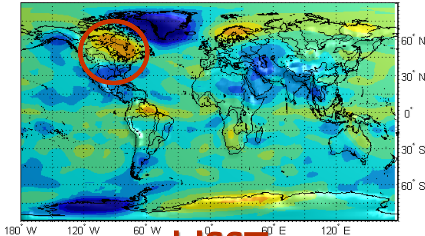
Trend in eq. water height [cm/year]
