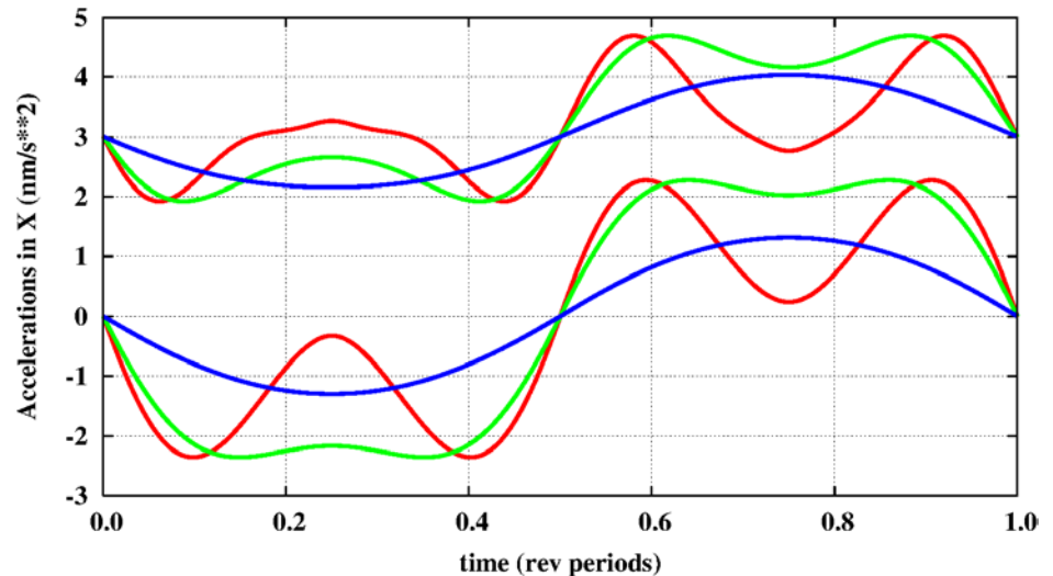
GPS Block IIA, X Accelerations
