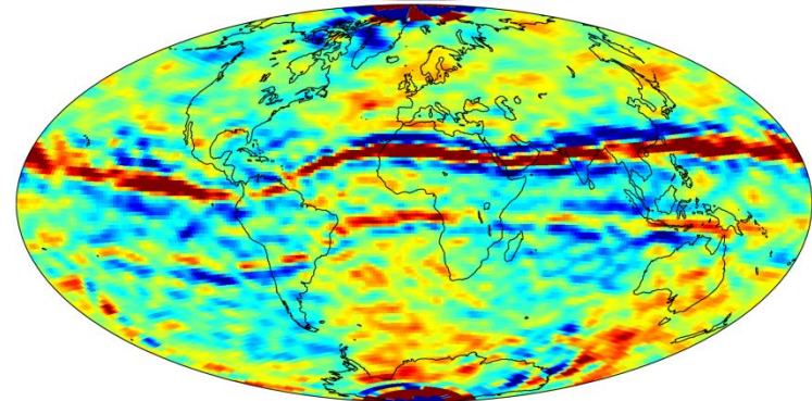
Geoid height differences (-5 cm ... 5 cm); Nov–Dec 2011
