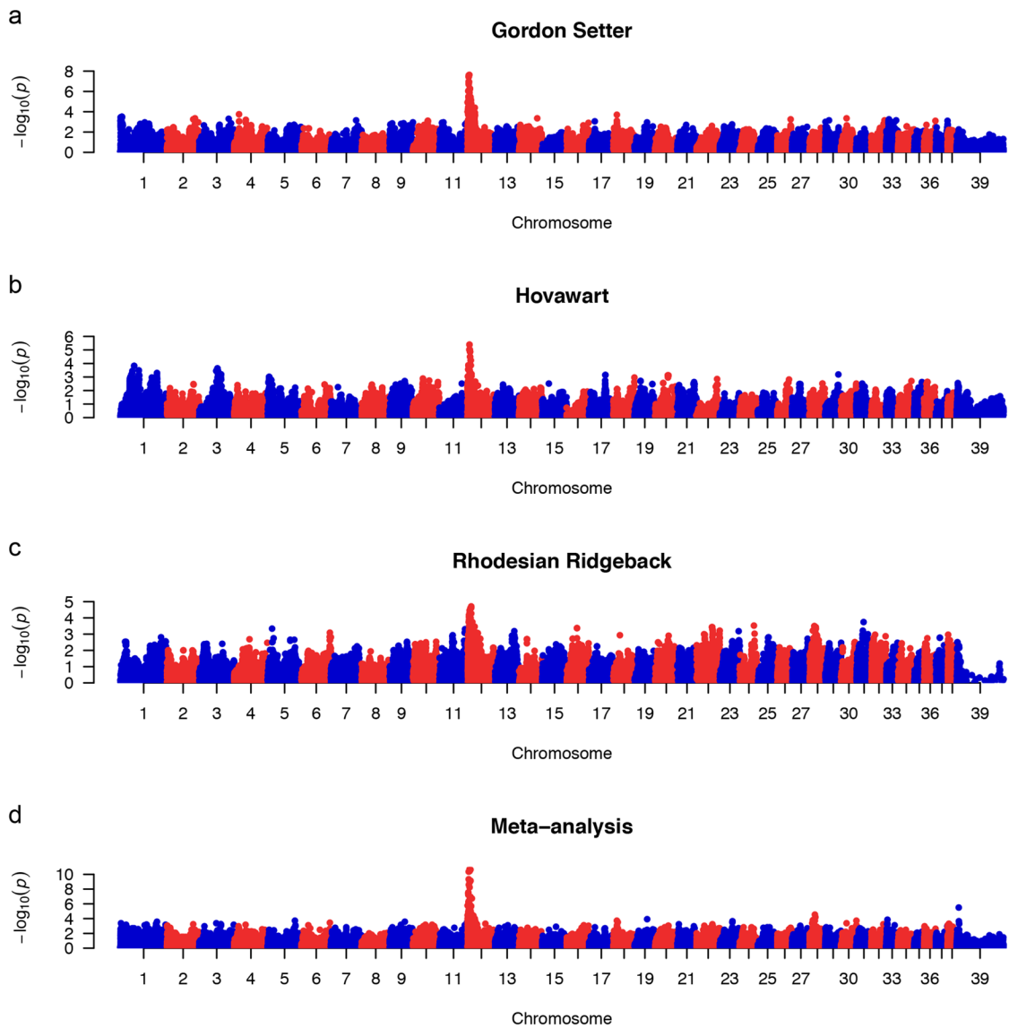
Fig 2. Manhattan plots showing a common peak on CFA12 in (a) GS p_{\text{raw}} = 2.4 \times 10^{-8} , (b) HV p_{\text{raw}} = 4.2 \times 10^{-6} , (c) RR p_{\text{raw}} = 2.0 \times 10^{-5} and (d) multi-breed meta-analysis p_{\text{raw}} = 2.1 \times 10^{-11} .
