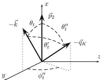
Fig. 20 Vectors and angles in the t -channel centre-of-mass frame
