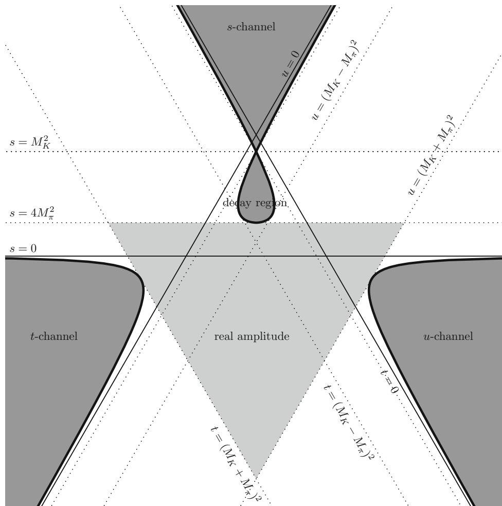
Fig. 1 Mandelstam diagram for $K_{l4}$ for the case $s_\ell = 0$
