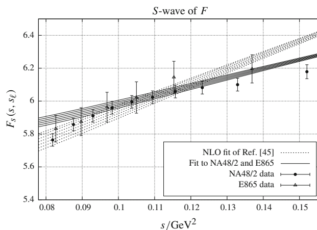
Fig. 12 Comparison of different fits for the S -wave of the form factor F : NA48/2 threshold parameter fit of [45] and a fit to the full data set. The (s, s_{\ell}) -phase space is projected on the s -axis. No isospin corrections are applied
