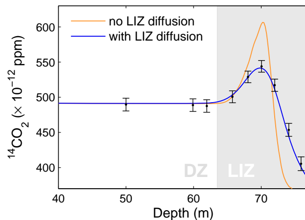
Fig. 6. Modeled ^{14}\text{CO}_2 profiles both with, and without diffusivity in the LIZ. Calculations done with the CIC firn air model.
