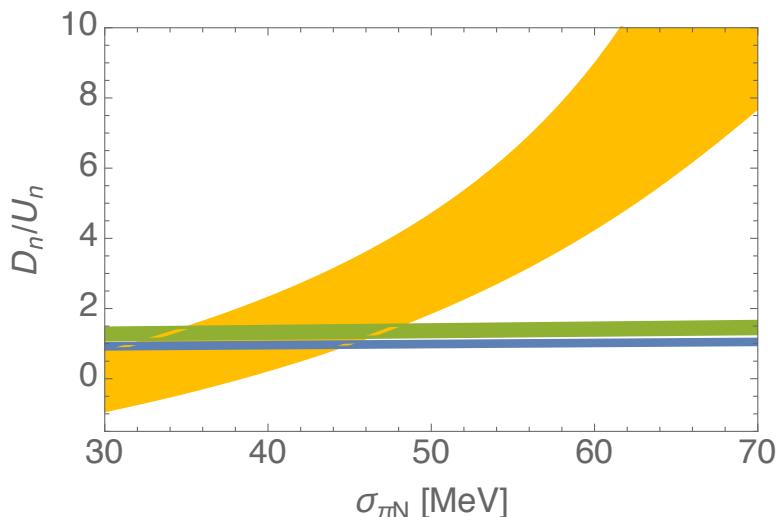
Figure 7. Dependence on \sigma_{\pi N} in the ratio of the hadronic terms U_N and D_N pre-multiplying the up- and down-type Wilson coefficient for h, H exchange (3.6). Shown is the case for N = \text{neutron} , with similar results obtained for N = \text{proton} . Color coding as in figure 6.
