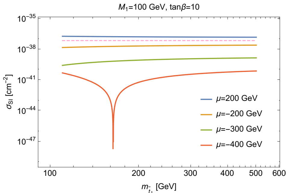
Figure 12. SI \chi -xenon cross sections as a function of the lightest stop mass m_{\tilde{t}_1} . The solid lines correspond to different values of the Higgsino mass \mu , while the pink dashed line is the existing limit from LUX. The blind spot at m_{\tilde{t}_1} \simeq 160 GeV is shown in red.
