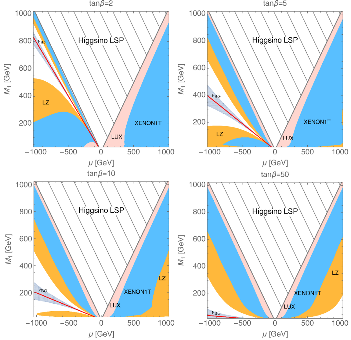
Figure 4. Current and projected limits on SI \chi -xenon scattering due to h exchange with \tan\beta = 2 (top left), 5 (top right), 10 (bottom left), and 50 (bottom right). The pink band shows the existing constraints from LUX [21], while projected limits from XENON1T [22] and LZ [23] are given by the blue and orange regions respectively. The blind spot where the SI cross section vanishes is denoted by the red line and lies within the irreducible neutrino background ( \nu_{BG} ) shown in gray. We assume the LSP is bino-like (figure 3), so do not consider the triangular, hatched region where \mu < M_1 and \chi becomes Higgsino-like.
