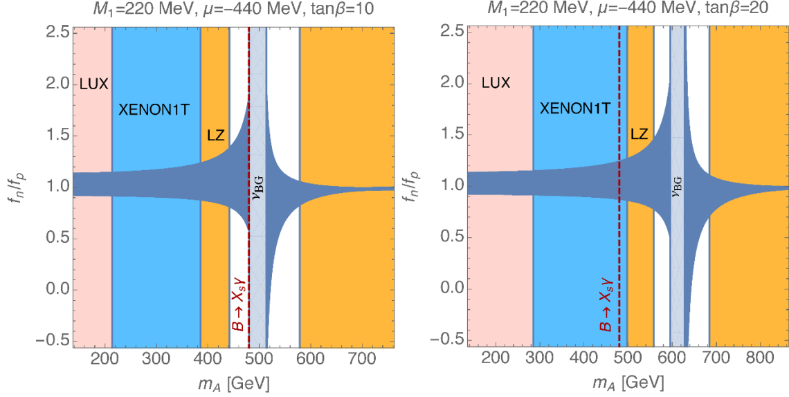
Figure 11. Current and projected results for the measure f_n/f_p of isospin violation arising from h, H exchange in SI \chi -xenon scattering for \tan\beta = 10 (left) and 20 (right). The dark blue region denotes the uncertainty on f_n/f_p as determined by Method 1. The existing and projected experimental limits are color coded as in figure 4, with the irreducible neutrino background ( \nu BG) shown by the central gray band. The region to the left of the dark red dashed line at m_A \simeq 480 GeV is excluded by B \rightarrow X_s \gamma [154].
