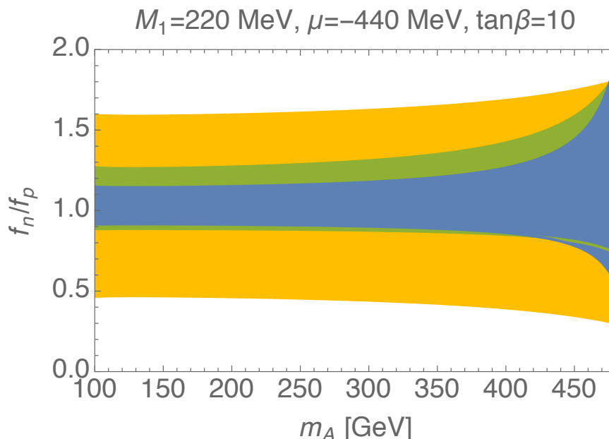
Figure 10. Amount of isospin violation in terms of f_n/f_p due to h, H exchange in \chi -xenon scattering. The shaded regions show the uncertainty on f_n/f_p due to each determination of the scalar matrix elements listed in section 2.1. Color coding as in figure 6.
