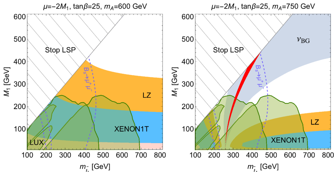
Figure 15. Current and projected limits in the (m_{\tilde{t}_1}, M_1) plane from h, H and \tilde{t}_{1,2}, \tilde{b}_L exchange in \chi -xenor scattering. In the figures, the value of m_A is increased for fixed \tan\beta . Excluded regions are color-coded as in figure 14, with B \rightarrow X_s\gamma ruling out both values of m_A entirely.
