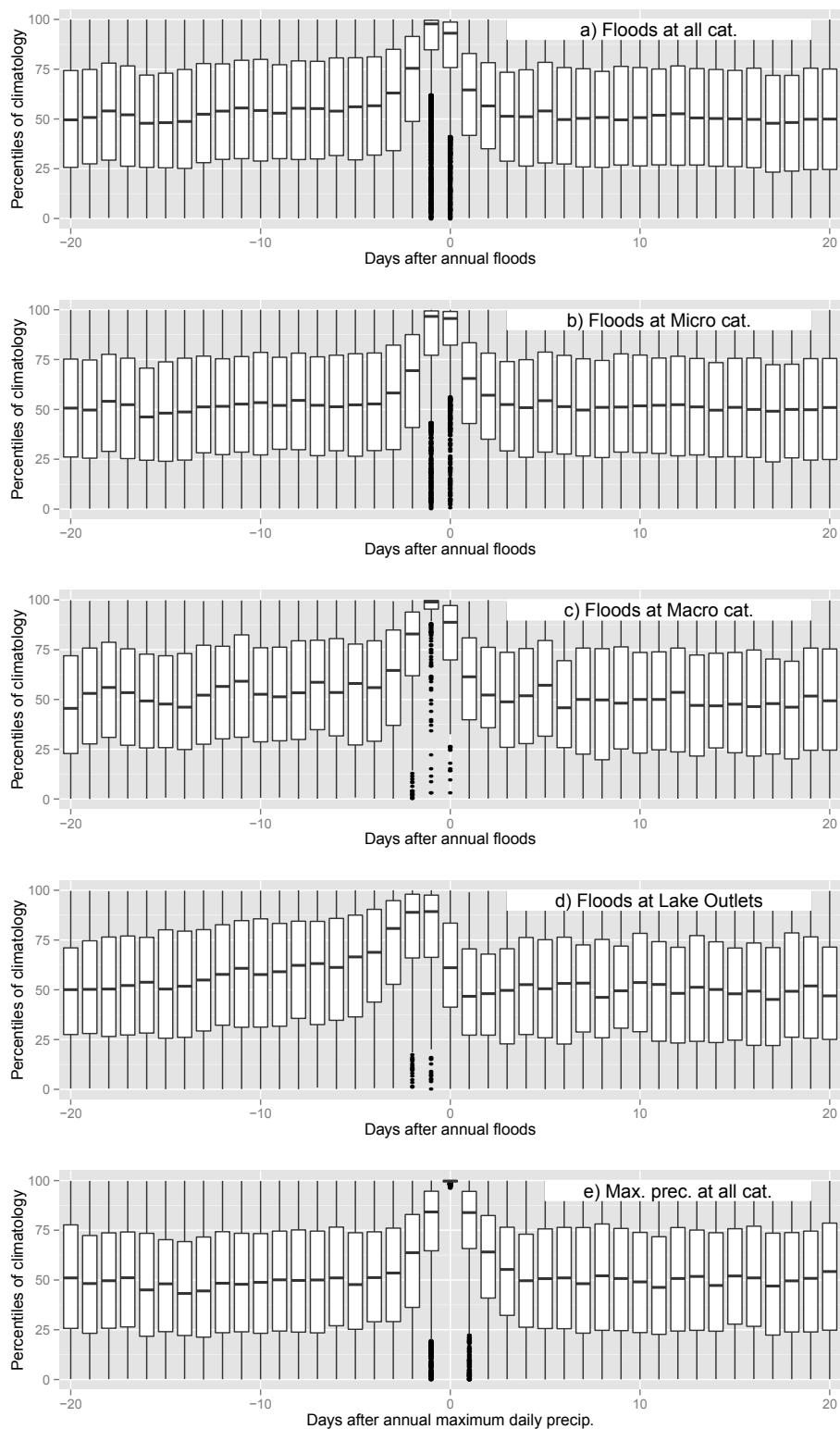
Figure 2. The distribution of daily precipitation before and after all flood events is shown in (a). For example, the boxplot at x \text{ D} \square 10 represents the distribution of daily precipitation percentiles 10 days prior to the 4257 annual flood events analyzed in this study (all HQs from all catchments). The middle line of the boxplots shows the median, the boxes comprise the 25–75 percentile range, and the whiskers end at a deviation from the mean of 1.5 the interquartile range. (b)–(d) Same as (a) but for floods in Micro catchments, Macro catchments and Lake Outlets. (e) The same procedure as in (a), but applied to annual maximum precipitation days instead of annual flood days.
