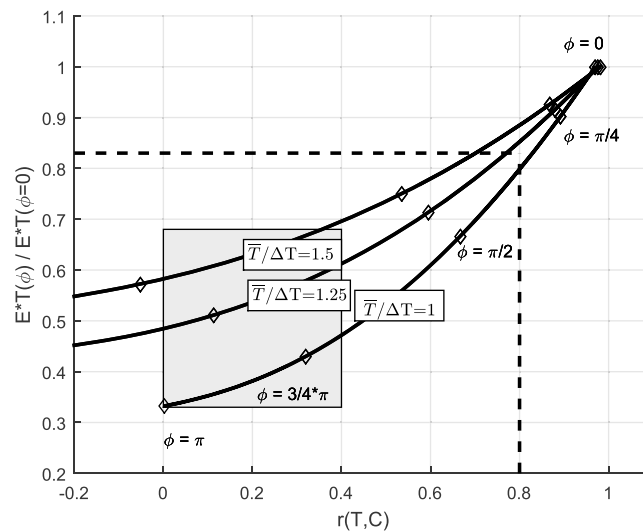
Figure 8. Product of transport efficiency T and source emission strength E ( E \cdot T(\phi) / (E \cdot T(\phi=0)) ) versus correlation coefficient r between dust concentration in the ice core C and transport intensity T for different \phi and different \bar{T}/\Delta T (equation (4)). This figure illustrates the reduction of dust in the ice due to a phase shift between maximum transport efficiency and the maximum of source emission strength. The dashed lines illustrate the mean correlation coefficient of CPP and dust concentration during the glacial. The grey square gives the range of respective correlation coefficients during the Holocene.
