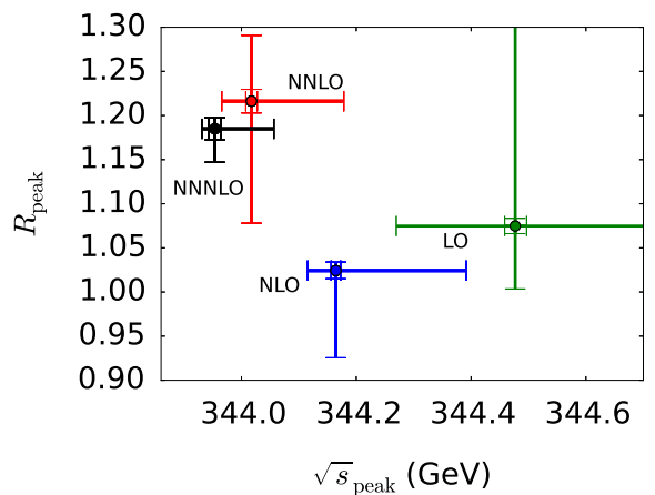
FIG. 3. Position and height of the cross section peak at LO, NLO, NNLO and N^3 LO. The unbounded range of the LO error bars to the right and up are due to the fact that the peak disappears for large values of the renormalization scale.
