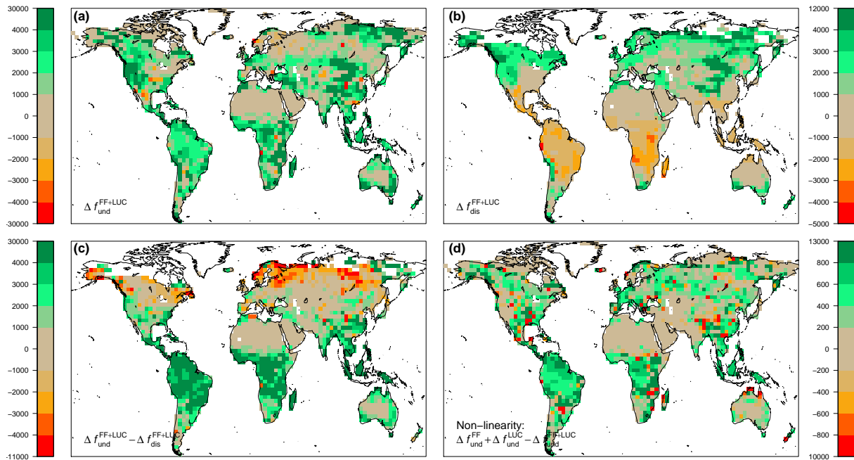
Figure 4. Top row panels: cumulative atmosphere-land C flux ( \text{kgCm}^{-2} ) induced by environmental change from 1700 to 2100 on undisturbed (a) and disturbed land (b; mean of cropland and pasture, weighted by respective area shares). Here, “disturbed” is approximated by cropland and pasture area (small at 1700), and “undisturbed” by natural area. The period 2005–2100 follows the RCP8.5 scenario. Climate and \text{CO}_2 are prescribed from the outputs of the coupled simulation (offline simulation F_0^{\text{FF}+\text{LUC}} uses outputs from F_{\text{LUC}}^{\text{FF}+\text{LUC}} ). (c) Difference of flux occurring on undisturbed and disturbed land f_{\text{und}}^{\text{FF}+\text{LUC}} - f_{\text{dis}}^{\text{FF}+\text{LUC}} . (d) Spatial distribution of synergy effects, cumulative in year 2100. Its global total over time is expressed also in Fig. 1 (difference between black and red curves).
