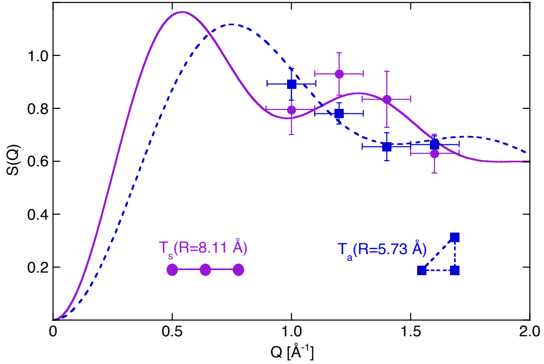
FIG. 3 (Color online) Q-dependence of the structure factor S(Q) for \text{Mn}^{2+} trimer transitions with \Delta S_{13}=\pm 1 for straight ( T_s ) and angled ( T_a ) trimer geometries shown in the insert. The data correspond to the results obtained for \text{KMn}_{0.10}\text{Zn}_{0.90}\text{F}_3 .
