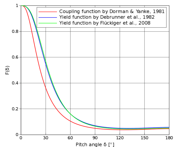
Figure 2. Deduced pitch angle distributions during the GLE on 13 December 2006 for the time interval 0305-0310 UT by using different NM response functions.
