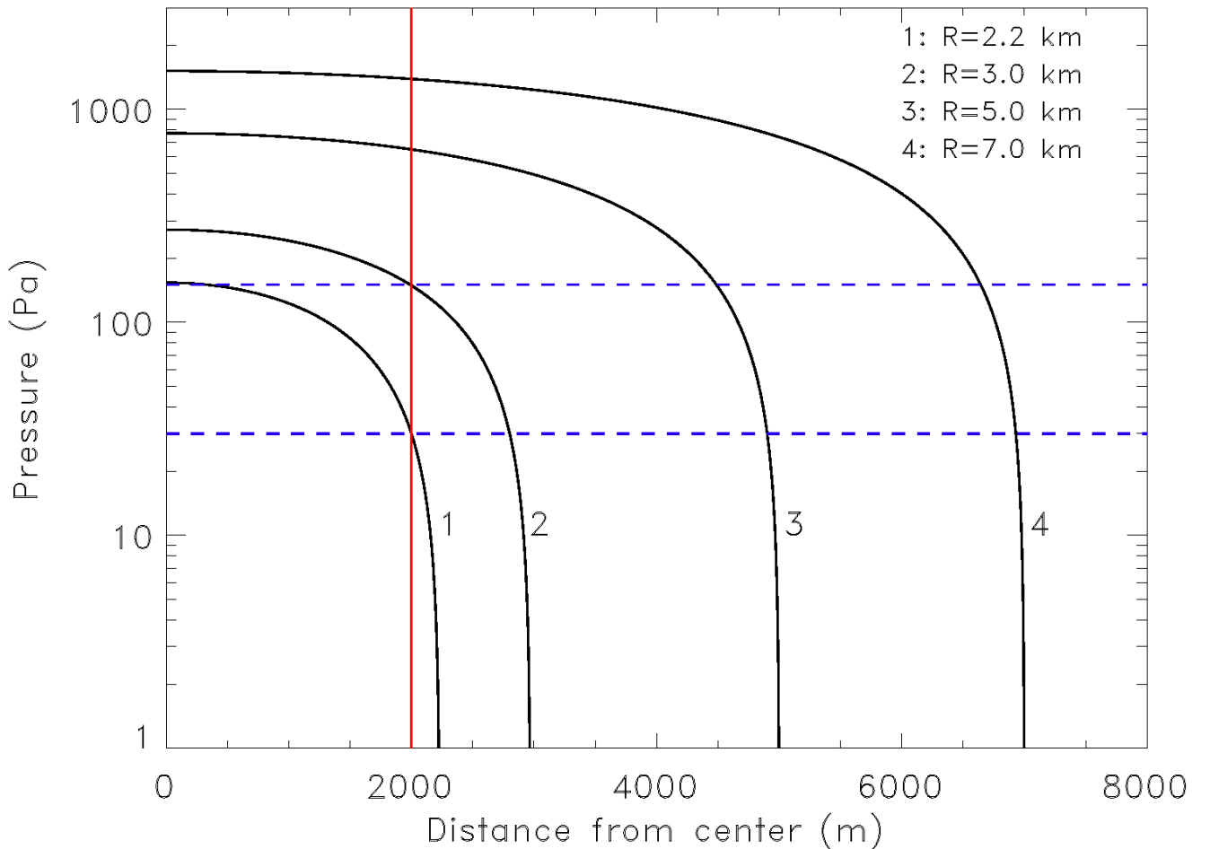
Fig. 15. Pressure versus depth inside the nucleus, for different initial sizes of the nucleus (radius R=2.2, 3.0, 5.0 or 7.0 \text{ km} ). The pressure increases with depth. The blue range corresponds to the best value of 30\text{--}150 \text{ Pa} for the compressive strength of the surface materials we see today ( 30\text{--}150 \text{ Pa} ). The red line at 2 \text{ km} indicates the current size of the nucleus, which is what we see today. For an initial radius of 2.2\text{--}3.0 \text{ km} , slightly larger than today, the pressure inside the nucleus exceeds the compressive strength of the layers we see today.
