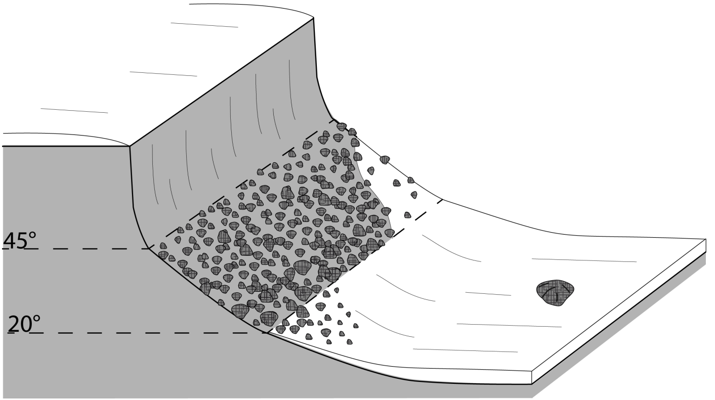
Fig. 8. Sketch of the general pattern in terms of relation between gravitational slopes and terrain morphologies: i) low-slope terrains ( 0-20^\circ ) are covered by fine material and contain a few large ( >10 m) and isolated boulders, ii) intermediate-slope terrains ( 20-45^\circ ) are mainly fallen consolidated materials and debris fields, with numerous intermediate-size boulders from <1 m to 10 m for the majority of them, and iii) high-slope terrains ( 45-90^\circ ) are cliffs that expose a consolidated material and do not show boulders or fine material. The borders between low- and intermediate-slope terrains are not always sharp (see text for details).
