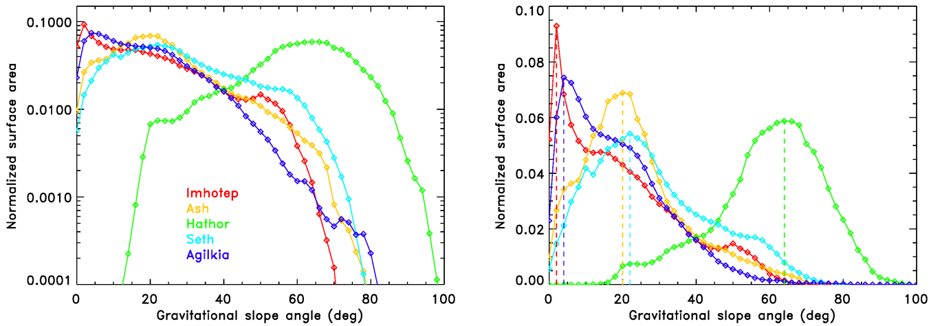
Fig. 6. Histogram of gravitational slope angles for the five regions, with one color per region, in logarithmic scale ( left ) and linear scale ( right ) for the Y axis. The values are normalized so that the sum of all Y values equals 1. Each region has a unique distribution of gravitational slopes, related to its unique topography. All regions cover a wide range of slopes from 0^\circ to almost 100^\circ . The gravitational slopes were derived from the SPC shape model (Jorda et al. 2015).
