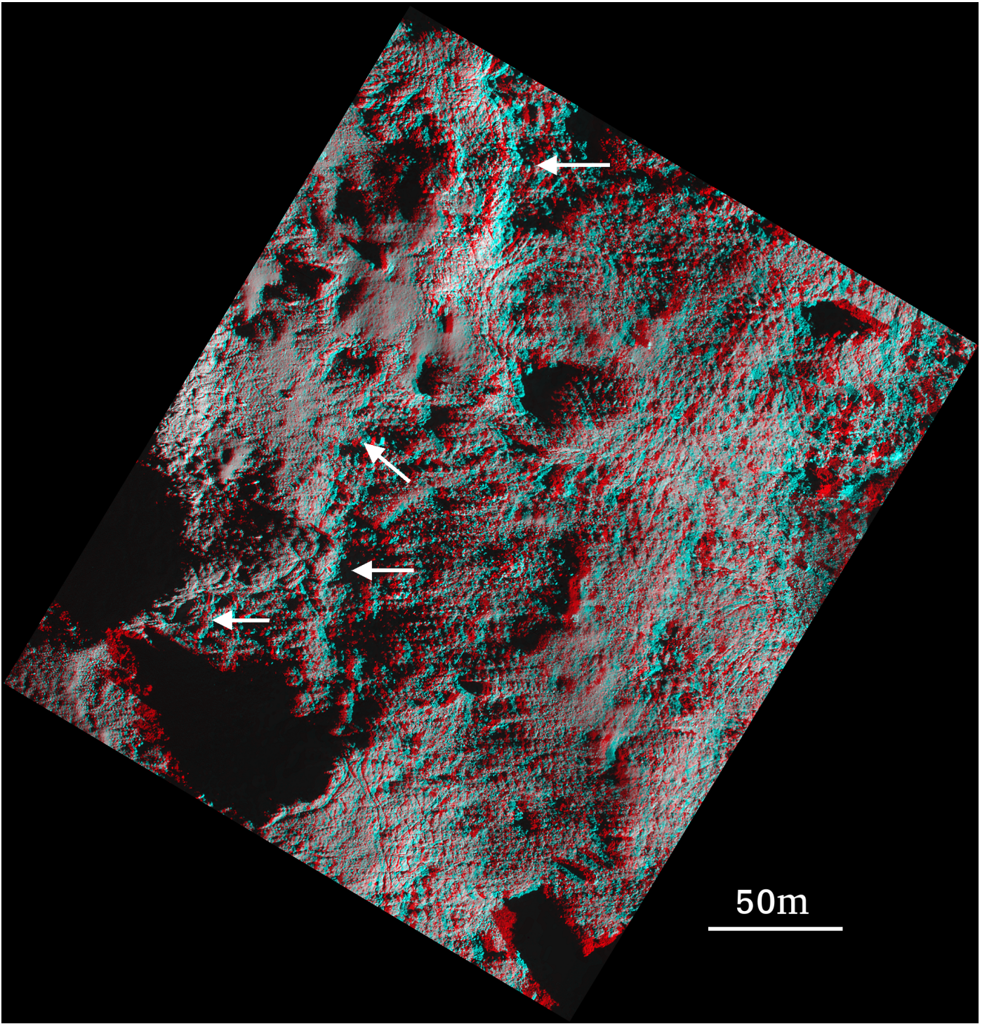
Fig. 11. Red/blue anaglyph of overhangs at a high spatial resolution of 18 \text{ cm pix}^{-1} , in the Maftet region. Several overhangs are visible in this anaglyph; they are indicated by white arrows, all with a length of \sim 10 \text{ m} and a height of \sim 5 \text{ m} . Image NAC_2014-10-19T13.18.55 (spatial resolution: 0.18 \text{ m pix}^{-1} ).
