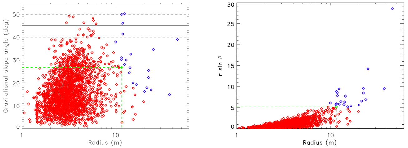
Fig. 13. Left panel: size (radius r ) of 2207 boulders of the Imhotep region as a function of their gravitational slope angle \theta (adapted from Auger et al. 2015). The black horizontal lines correspond to the angle of repose \theta_{\text{repose}} = 45 \pm 5^\circ ; there are no boulder on slopes larger than the angle of repose. Right panel: value r \sin \theta for each boulder, as a function of its radius. Both panels: for robustness, we rejected the upper 1% of the r \sin \theta distribution (blue points). For the remaining 99%, the boulder with the highest value r \sin \theta is highlighted in green and corresponds to r = 11.5 m and \theta = 26.8^\circ , as indicated by the green horizontal and vertical dashed lines.
