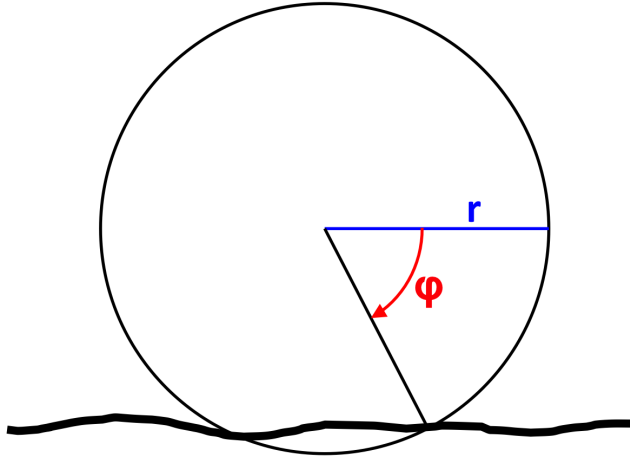
Fig. 12. Scheme of a boulder lying on the surface. The radius of the boulder is r , and its contact area with the surface is defined by the angle \varphi .
