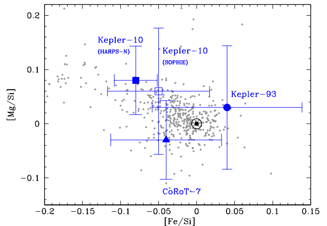
Figure 1. [Mg/Si] vs. [Fe/Si] for the studied stars, together with the comparison dwarf (gray small dots) from Adibekyan et al. (2012b) with T_{\text{eff}} = T_{\odot} \pm 300 K. The position of the Sun is shown for comparison.
