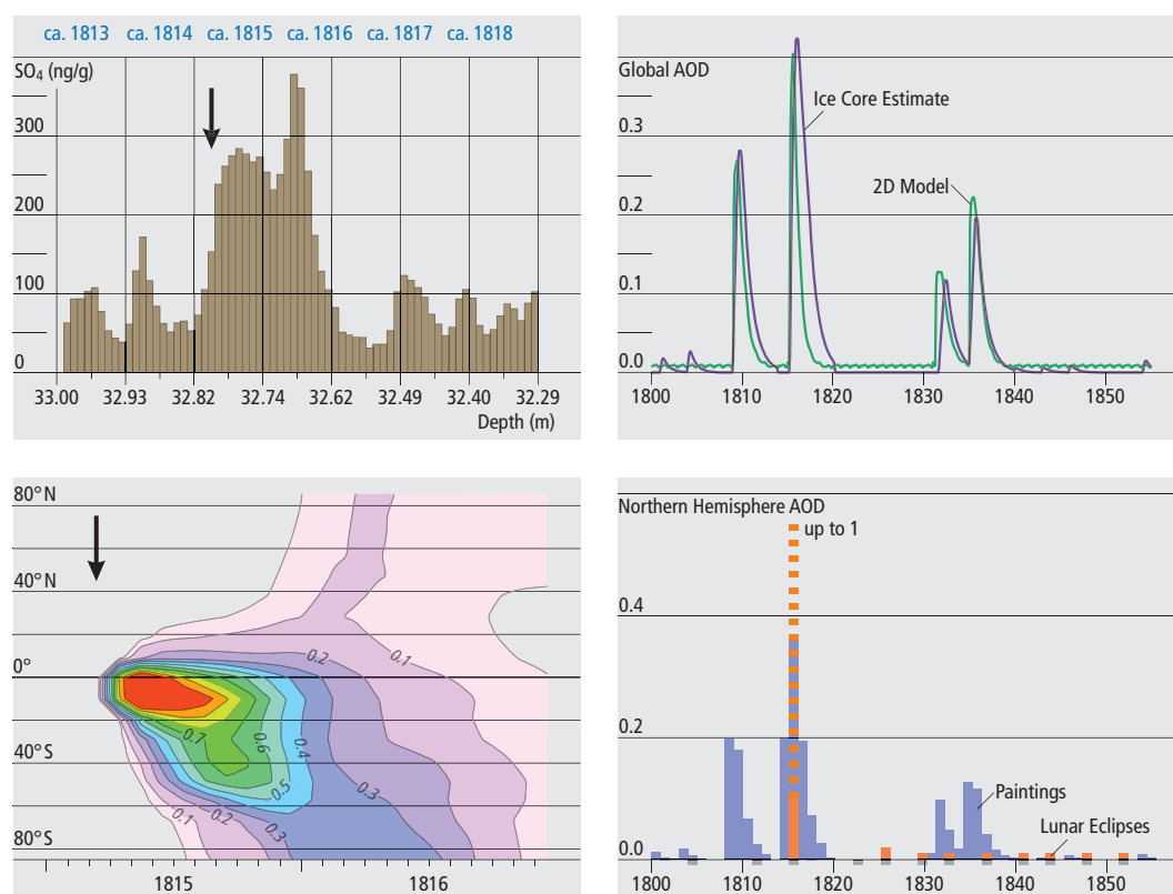
Fig. 6. (Top left) Sulphur concentration in segments of an ice core from Greenland. 38 (Top right) Reconstruction of global aerosols optical depth from ice cores using statistical techniques 39 or a 2D aerosol model. 40 (Bottom left) Spread of the aerosols (zonally averaged aerosol optical depth) after the Tambora eruption in a 2D aerosol model. 41 (Bottom right) Estimated aerosol optical depths from paintings 42 and lunar eclipses 43 (grey indicates observed eclipses). The arrow indicates the eruption of Tambora.
