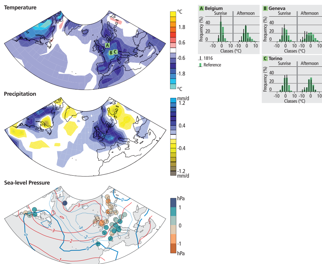
Fig. 10. Climate in summer (Jun–Aug) 1816 expressed as anomalies from a contemporary reference observations period (1799–1821). Shown are reconstructions 92 of (top) temperature (right: frequency distributions of daily temperature anomalies from three stations), (middle) precipitation and (bottom) sea-level pressure (black contours, in hPa). Dots show the standard deviation of daily sea-level pressure, 3–6 day band-pass filtered 93 and expressed as anomalies from a present reference (1981–2010, red contours, in hPa).
