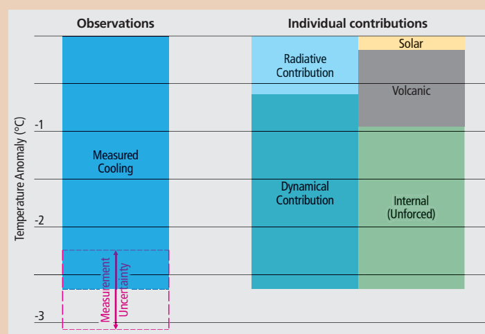
Contributions of direct and indirect Tambora effects and of internal (unforced) variability to the temperature anomaly in the summer of 1816 in Geneva. The quantification is based on the observed diurnal temperature range on clear sky days as well as model results. 108
