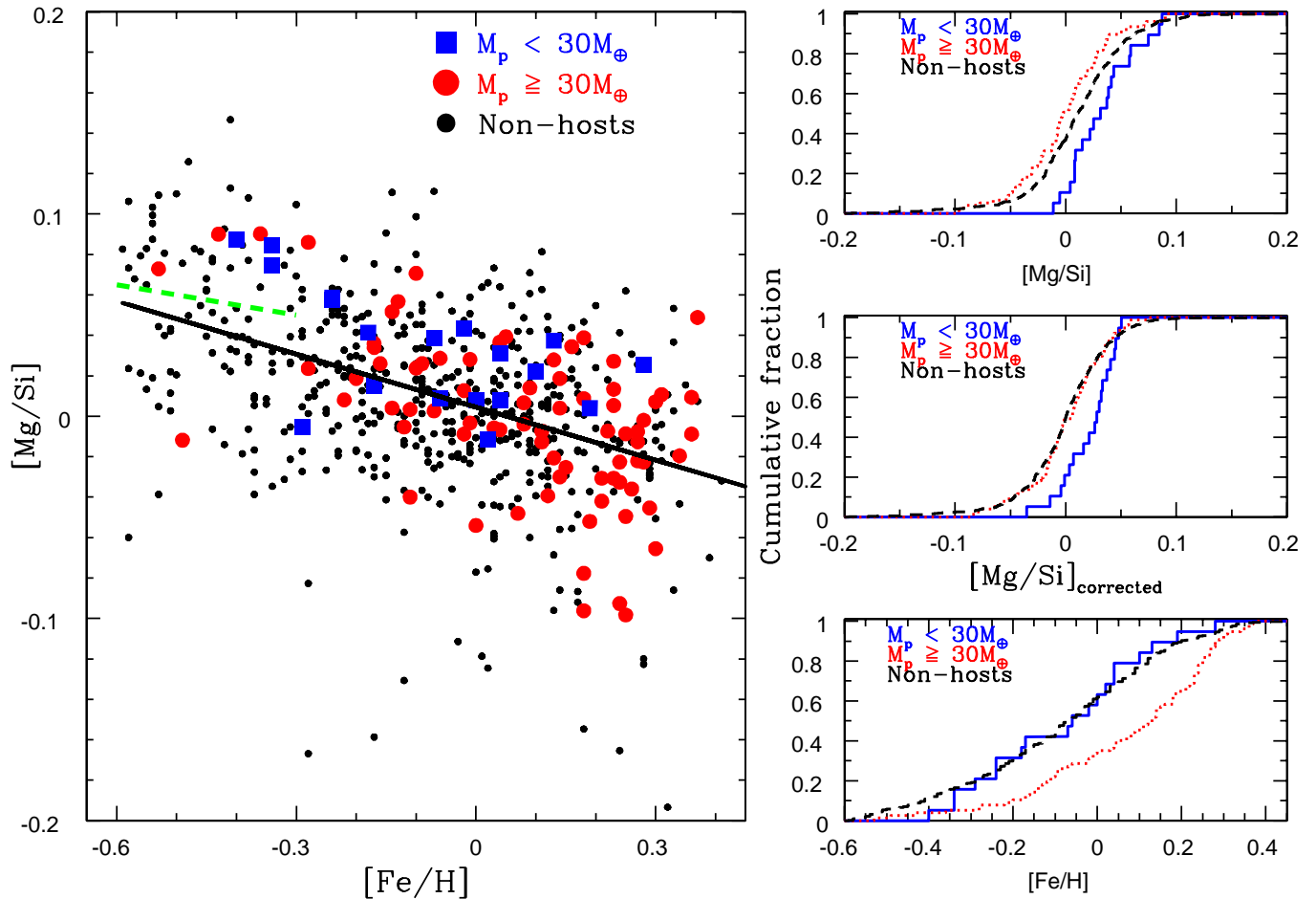
Figure 1. Left. [\text{Mg}/\text{Si}] versus [\text{Fe}/\text{H}] for stars without detected planets (black dots), stars hosting low-mass planets (blue squares), and stars hosting high-mass planets (red filled circles). Cumulative distribution of [\text{Mg}/\text{Si}] ( top right ), [\text{Mg}/\text{Si}] after correcting for the Galactic chemical evolution ( middle right ), and [\text{Fe}/\text{H}] ( bottom right ) for stars with and without detected planets. The black solid line provides linear fit to all the data points and the green dashed line shows separation between Galactic thin- and thick-disk stars.
