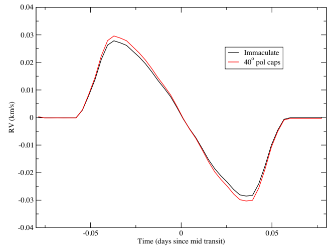
Figure 3. Simulation of the Rossiter-McLaughlin effect on a star similar to WASP-80. Two configurations are tested here. One where the star has no spots, and one where it possesses spots at the poles covering the upper and lower 40 degrees in latitude. This increases slightly the amplitude of the effect, because the fractional contribution to the stellar rotation hidden by the planet has gained in importance.
