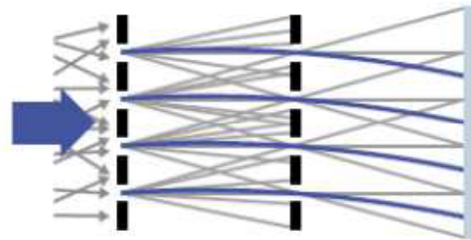
Figure 3 – The moiré deflectometer. The trajectories of undisturbed particles (grey lines) are modified by the presence of a force (blue lines) and a shift of the fringe pattern occurs (reprinted figure from ref. 37. Copyright (2014) by Macmillan Publishers Limited. DOI: 10.1038/ncomms5538).
