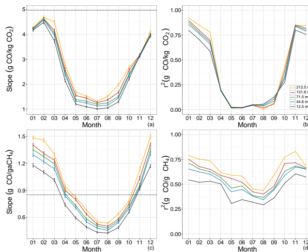
Figure 2. Slope and r^2 for \Delta\text{CO} / \Delta\text{CO}_2 (a, b) and \Delta\text{CO} / \Delta\text{CH}_4 (c, d) for the sampling levels 12.5 (black), 44.6 (blue), 71.5 (green), 131.6 (red) and 212.5 m (yellow). Horizontal dashed lines represent Swiss inventory estimates for 2013.
