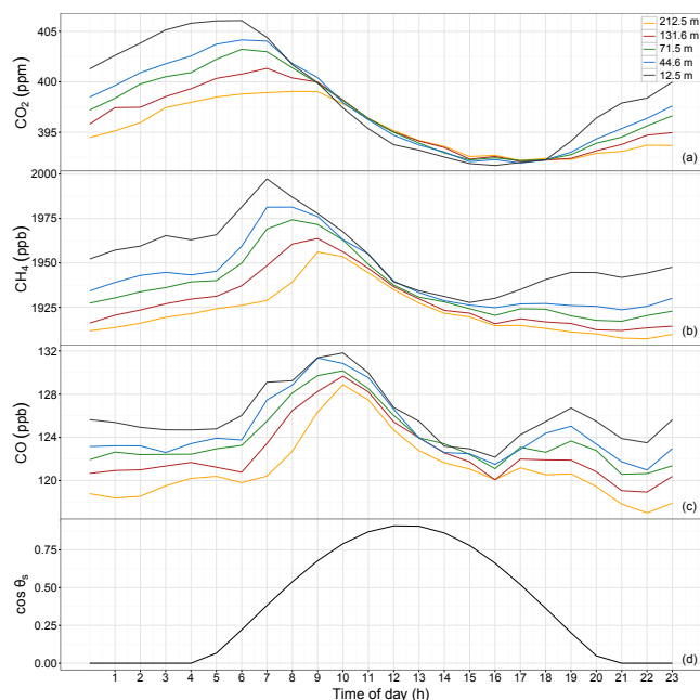
Figure 4. Mean diurnal cycles of CO 2 (a), CH 4 (b), CO (c) in June for the sampling levels 12.5 (black), 44.6 (blue), 71.5 (green), 131.6 (red), and 212.5 m (yellow) together with the cosine of the solar zenith angle ( \cos \theta_s ) calculated for the geographical coordinates of site Beromünster.
