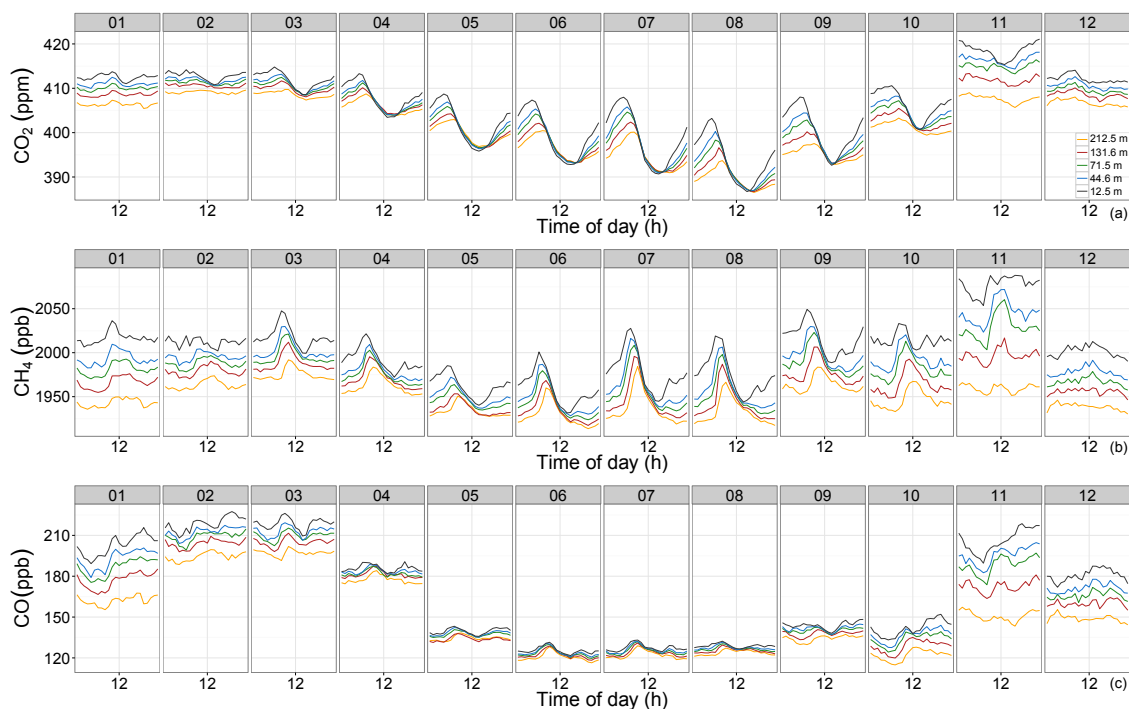
Figure 3. Monthly mean diurnal cycles of CO 2 (a), CH 4 (b) and CO (c) for the sampling levels 12.5 (black), 44.6 (blue), 71.5 (green), 131.6 (red), and 212.5 m (yellow). The x axis on each subplot is centered at noon (UTC 12:00).
