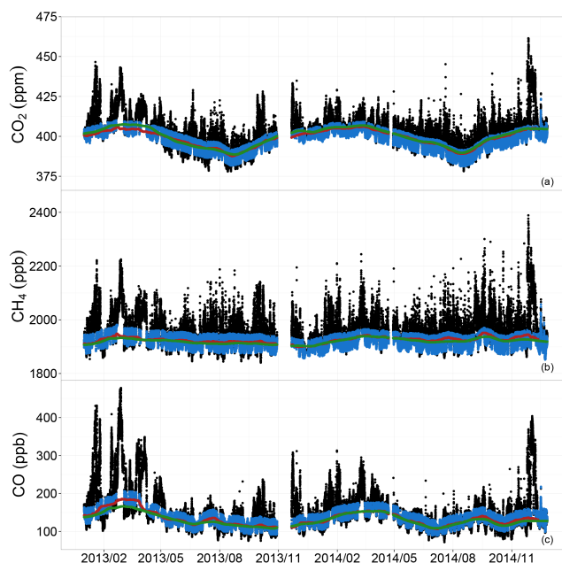
Figure 1. Time series (December 2012–December 2014) of CO 2 (a), CH 4 (b), and CO (c) at Beromünster for air sampled at 212.5 m. Color codes indicate the following: all measurements (black), estimated background values using 2\sigma filter (blue), moving average of 30 days based on the background estimates (red), and seasonal variations estimated by REBS (green).
