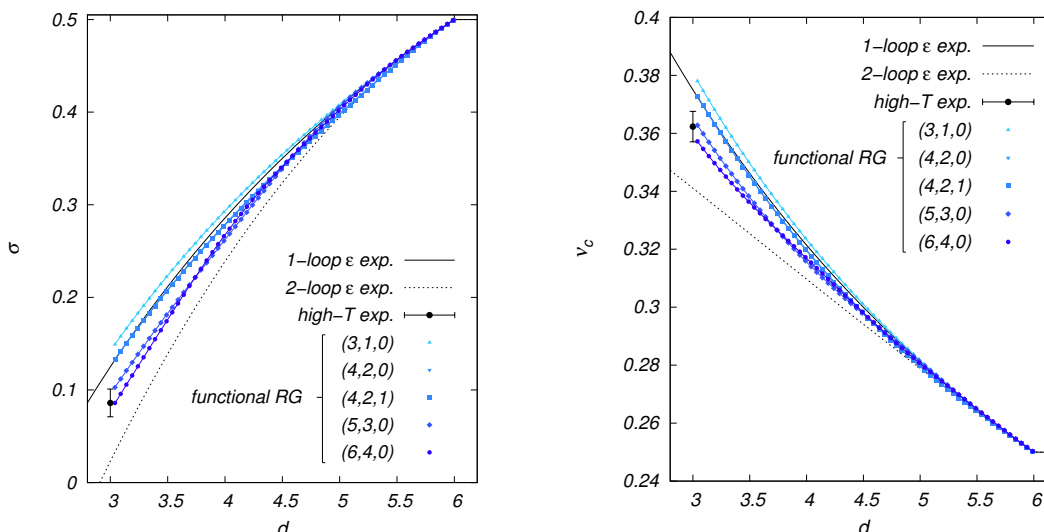
Figure 1. Critical exponents \sigma = 1/\delta and \nu_c as a function of Euclidean dimension d for different truncations of the scale-dependent effective action \Gamma_k , as specified by the set of integers (n_U, n_Z, n_W) [cf. section 4]. The data for the truncation (4, 2, 1) lies almost exactly on top of that for (4, 2, 0) . Shown in comparison are results from the one- and two-loop \epsilon expansion [20, 43] as well as high-temperature series expansion data ( d = 3 ) [20, 34]. We observe that the numerical accuracy of the functional RG results improves significantly as one goes to higher orders in the derivative and field expansion, respectively.
