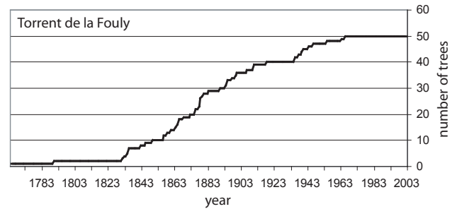
Fig. 5. Age structure of the trees sampled at Torrent de la Fouly. The oldest tree reached sampling height in AD 1765.
