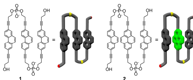
Figure 1. Chemical structure and illustrative model representations of trimers 1 and 2 . Pyrene is highlighted green.
