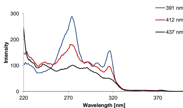
Figure 5. Excitation spectra of poly1 . Conditions: 1\ \mu\text{M} in 10 mM sodium phosphate buffer pH 7.0, 10% ethanol; \lambda_{\text{em}} 391 nm (blue), 412 nm (red) and 437 nm (black); excitation slit: 5 nm, emission slit: 5 nm.
