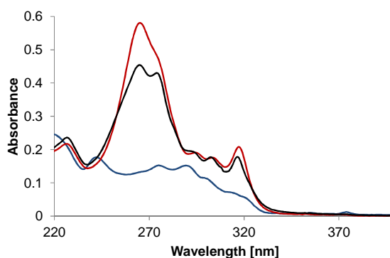
Figure 2. Absorption spectra of 1 in 10 mM sodium phosphate buffer pH 7.0, 10% ethanol (blue: at 20°C, red: at 80°C) and in ethanol at 20°C (black), concentration: 1 μM.
