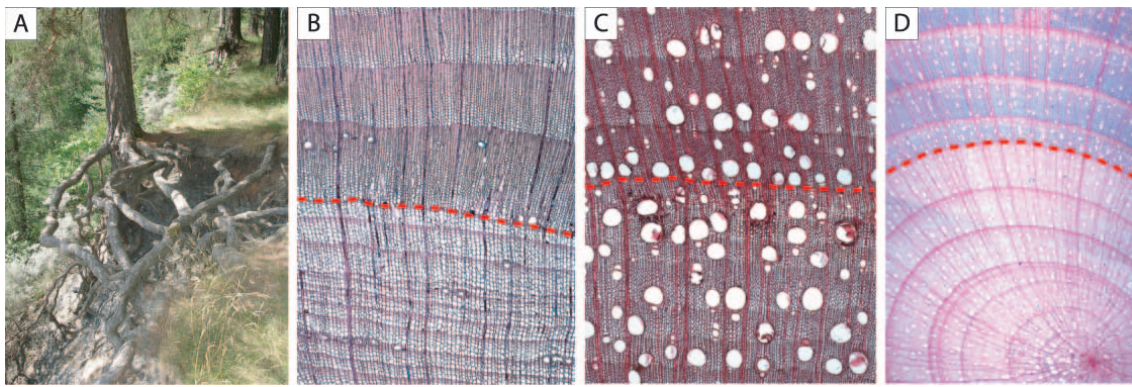
Fig. 6. (a) Exposed roots of Pinus sylvestris L. (b) In Abies alba Mill., larger increment rings with distinct latewood are formed after sudden exposure (dashed red line). (c) Following sudden exposure, the arrangement of vessels in Fraxinus excelsior L. change from diffuse-porous to ring-porous. (d) In addition to cell changes, tension wood is formed in this root of Acer pseudoplatanus L. (Source: Hitz, 2008).
