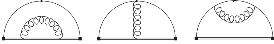
Figure 9. Diagrams obtained from eq. (7.3) at NLO. The double line is the fundamental Wilson line and the black squares are the insertion of the soft fermion fields.
