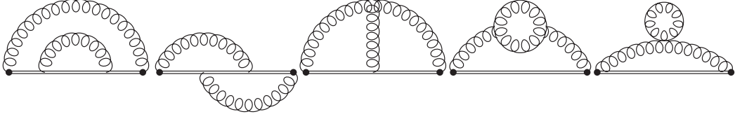
Figure 8. Diagrams contributing to \delta\hat{q}_L|_{\text{loop}} at NLO.
