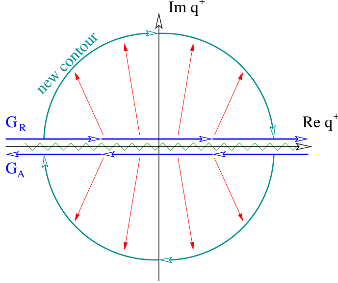
Figure 7. Integration contour in the complex q^+ integration, and the deformation we use to render q^+ \gg gT . G_R runs above the real axis and G_A below.
