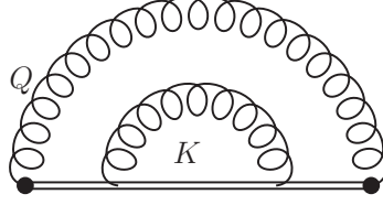
Figure 12. The rainbow diagram.
