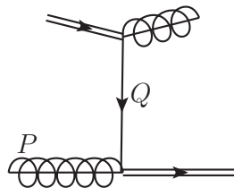
Figure 4. The soft limit of a t - or u -channel quark exchange diagram. P is the hard momentum and Q is the soft quark momentum.
