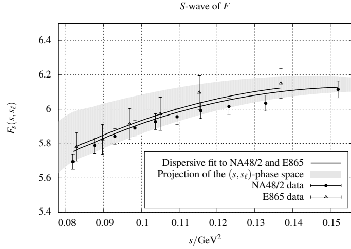
Figure 1: Fit result for the S -wave of the form factor F . The dispersive description reproduces beautifully the curvature of the form factor. The (s, s_\ell) -phase space is projected on the s -axis, the plotted lines correspond to splines through the (s, s_\ell) -values of the data sets with a single bin in s_\ell -direction.
