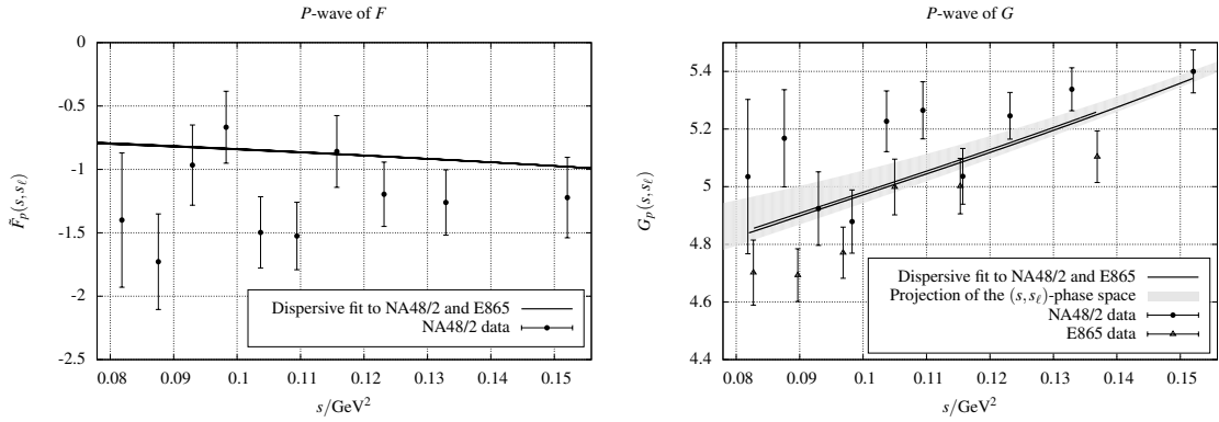
Figure 2: Fit results for the P -waves of the form factors F and G . The (s, s_\ell) -phase space is again projected on the s -axis.
