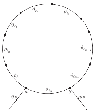
Figure 2. Auxiliary graph for the sum of internal twisting angles. The endpoints of each line correspond to vertices of the non-empty finite set \mathcal{V} of the abstract graph \mathcal{G} . Along the internal lines \ell_1, \dots, \ell_N flow twisting angles \vartheta_{\ell_1}^\mu, \dots, \vartheta_{\ell_N}^\mu . Along external lines flows the twisting angle \vartheta_P^\mu of the particle P under consideration.
