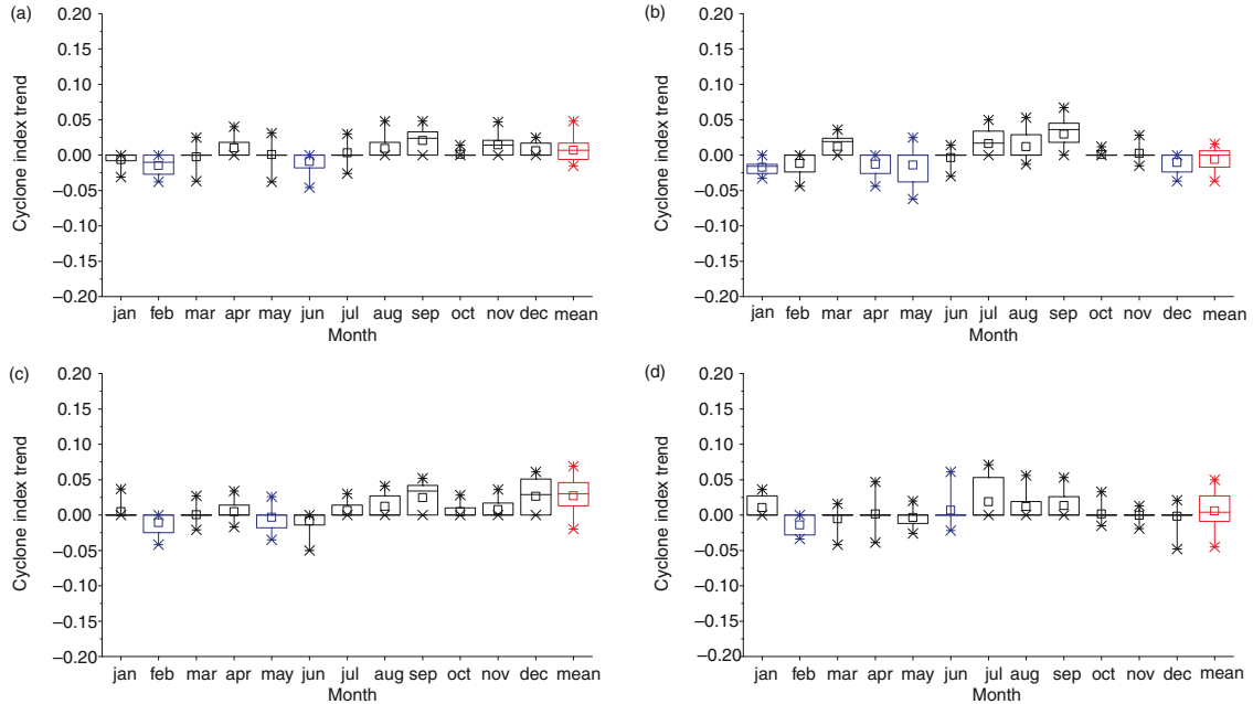
Fig. 12. Trends of the cyclone number index for the four sectors of the Mediterranean region. (a) NW, (b) NE, (c) SW, (d) SW. The red symbol on the right of the panels denotes the trend of the mean monthly cyclone number. Blue symbols denote months where at least 25% of CDTMs present statistically significant trends with the same sign.
