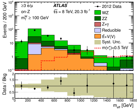
(e) \geq 3e/\mu , on-Z
