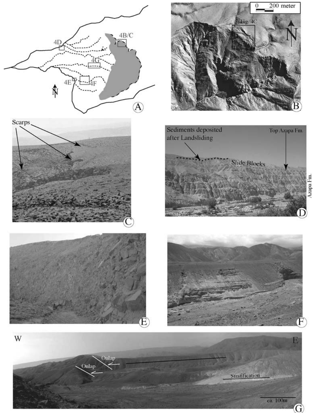
Fig. 4 a Overview of 'Lluta collapse' showing location of photos from the field, b rectified aerial photo, and c photo showing the headwaters with an en-echelon arrangement of incipient scarps (arrowed) forming a stair-case topography, d photo from the Lluta valley indicating the detachment horizon of the Lluta landslide, e slide block with brecciated ignimbrites, f horizontally stratified sediment dammed behind these blocks, and g onlap-relationship between stratified sediments and tilted slide blocks
