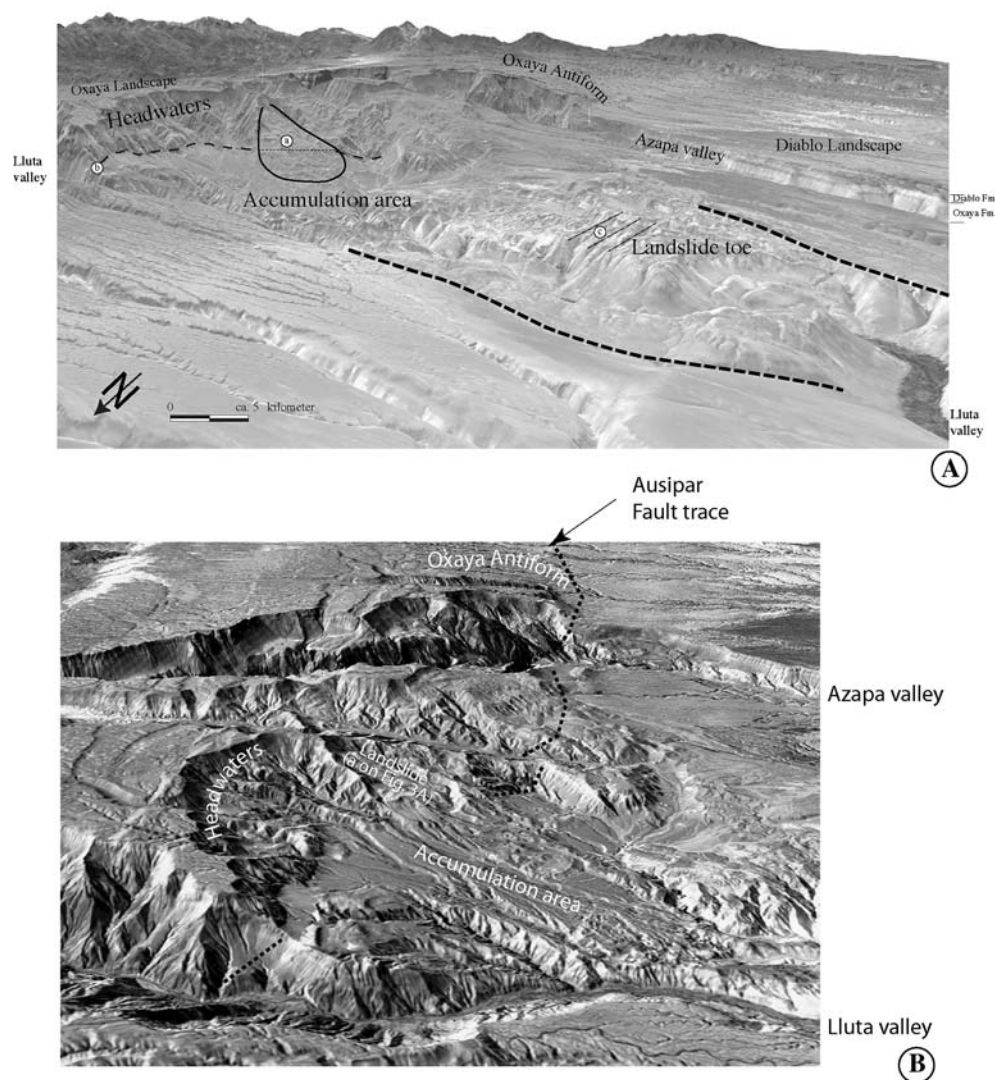
Fig. 3 a 3D visualization of a SRTM–DEM overlain by an autorectified LANDSAT 5 image showing the study area with its characteristic geomorphic domains. b displays a closer look to the headwaters and the accumulation area. Note the presence of a landslide mass that has not been completely removed
