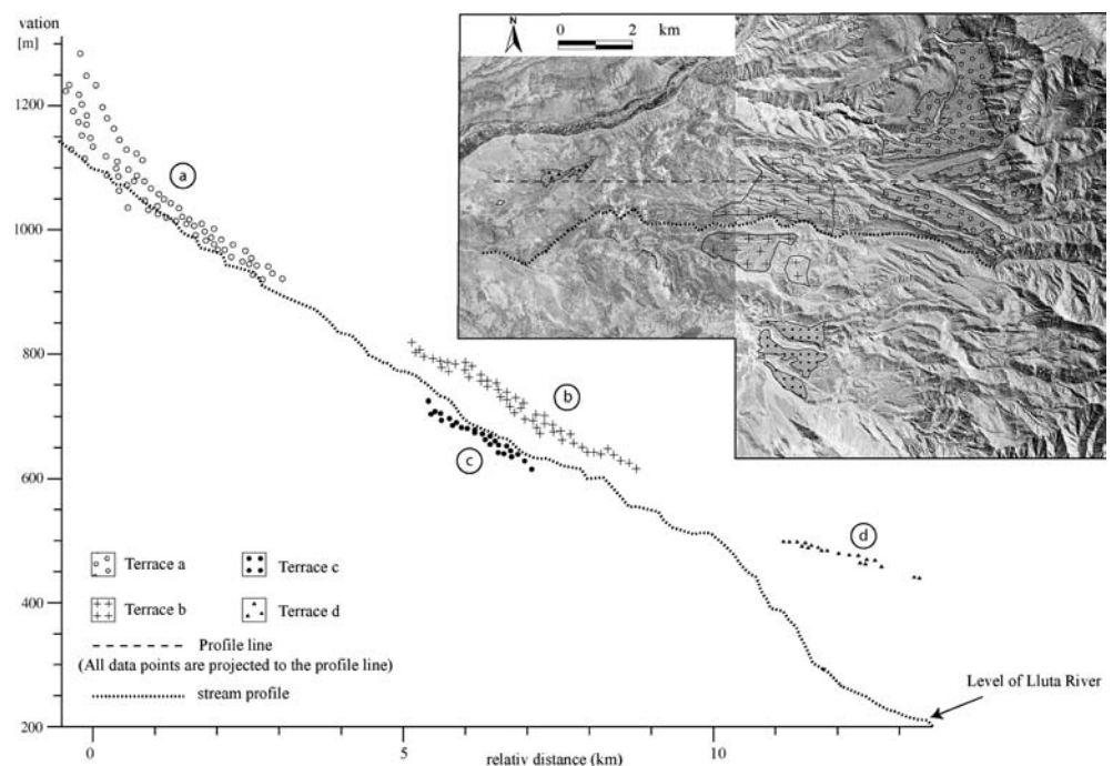
Fig. 10 Elevation profiles of four separately analysed terraces in the accumulation area of 'Lluta collapse'. All data points are projected to the profile line (see also bold line in Fig. 2 for localization of the profile). Vertical exaggeration is 10x. See text for further explanation. Note that the > 2.5 Ma-old exposure age was determined for terrace c, and that terrace d was deposited by the Lluta river
