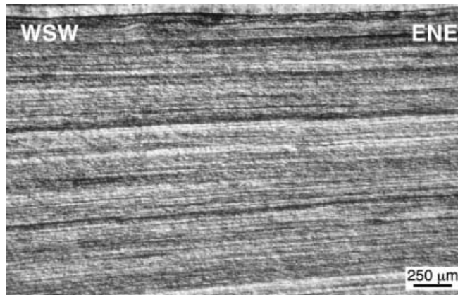
Fig. 7 Quartz fabric from Speikboden (locality L, Fig. 1). The dated pseudotachylyte of Fig. 8 was taken from the same outcrop. Foliation 341/37, lineation 030/28
