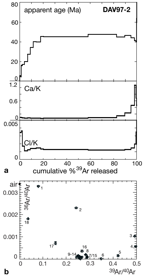
Fig. 13 a ^{40}\text{Ar} – ^{39}\text{Ar} stepwise-heating spectra, and b isochron diagram for pseudotachylyte DAV97/2 from Zinsnock (locality D). Located in the narrow gully above Haidacher Alm, at 2045 m altitude, 850 m SE of Zinsnock peak (see Fig. 12b)
