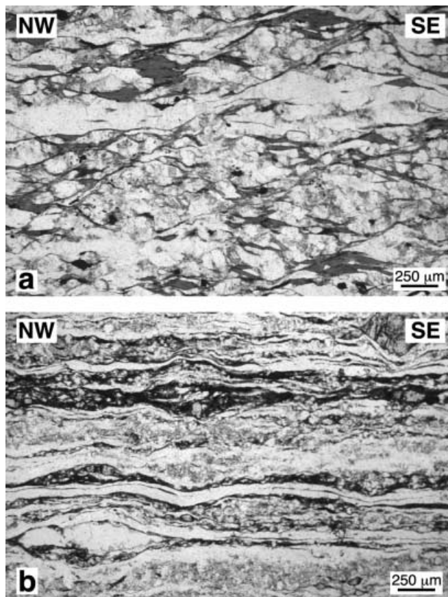
Fig. 15a, b DAV mylonites in the Weidental section (locality N, Fig. 1). a Typical sample from the southernmost outcrops just north of the Periadriatic fault. Coarse-grained quartz ribbons alternating with more feldspar-rich layers are typical and very similar to samples from the southernmost parts of the sections at Staller Sattel (C) and Zinsnock (D). Biotite is (at least initially) stable in the well-developed sinistral shearbands which are transitional to discrete brittle Riedel faults on both the thin-section and outcrop scale. Foliation 048/42 (backrotated between discrete sinistral Riedel faults), lineation 120/15. b Laminated finer-grained mylonite from the forestry road section further north, with alternating quartz ribbons (partially recrystallized, mainly by a subgrain rotation mechanism) and recrystallized feldspar layers. Garnet forms porphyroclasts and is often fractured to form bookshelf structures. Sinistral sense of shear is clear from these bookshelf structures in garnet and larger feldspar porphyroclasts, from strong preferred orientation and oblique grain fabrics in quartz and from shear bands, in which biotite is initially stable but is subsequently partially replaced by chlorite. Strong undulose extinction and deformation lamellae in quartz also argue for a retrograde deformation path. Foliation 002/45, lineation 264/02
