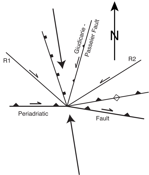
Fig. 5 Summary of fault orientations related to the dextral transpressive Periadriatic fault system from the Maults-Plattspitz-Ochsensprung area (original data in Stöckli 1995 and Grollimund 1996)
