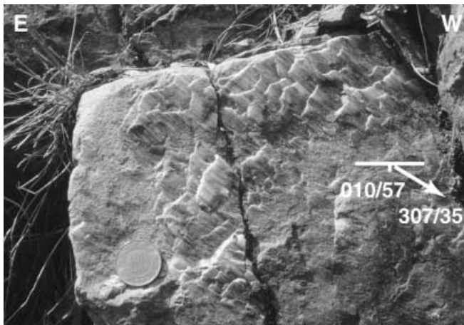
Fig. 6 Stepped slickenfibres indicating dextral transpressive reactivation of the southernmost limit to the DAV mylonites, south of Zinsnock (location D, Fig. 1)
