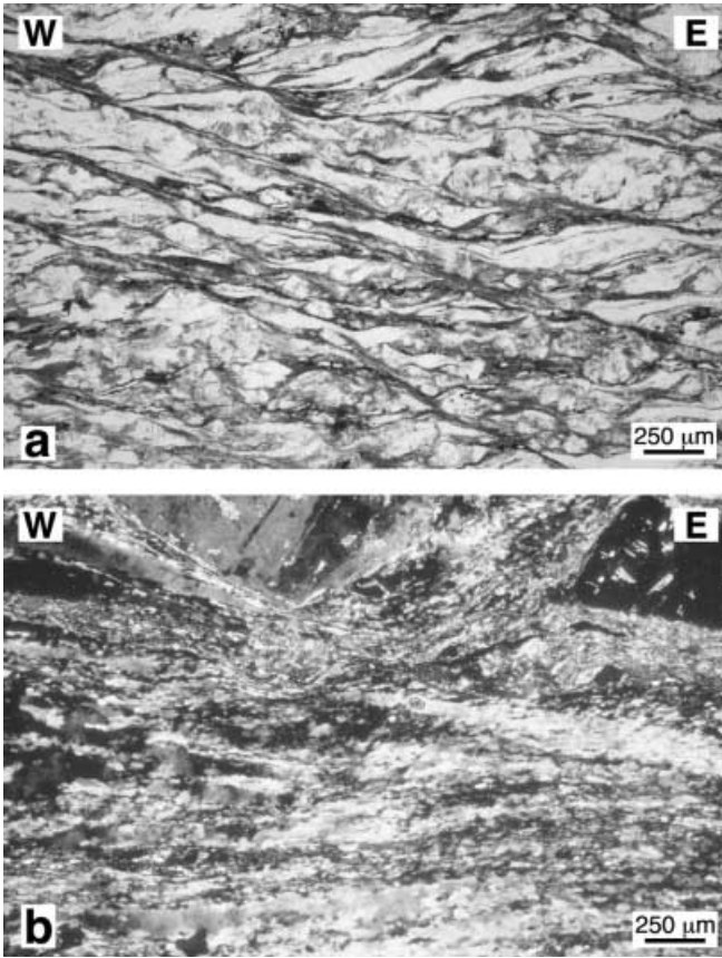
Fig. 4a, b Dextral overprint of the northern Rensen pluton contact near Plattspitz (Fig. 1; coordinates 1.697.190/5.193.250, 1:10,000 grid of South Tyrol, 2550 m elevation). Foliation 015/76, lineation 115/00. a Austroalpine from 20 cm north of the contact itself. b Adjacent mylonitized Rensen tonalite
