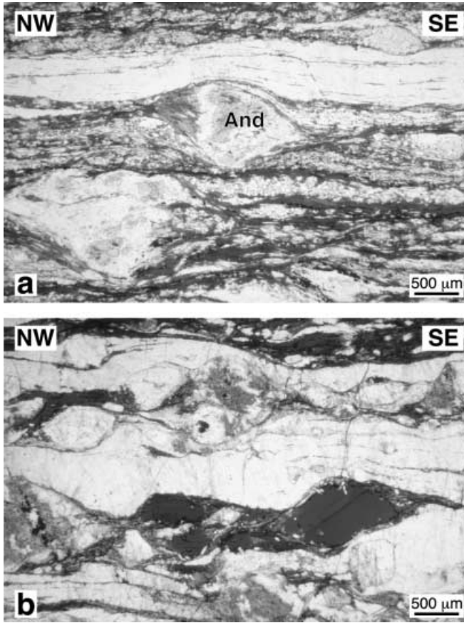
Fig. 10 a Sigmoidal andalusite porphyroclasts ( And ), indicating sinistral shearing, with new biotite and muscovite growth in the pressure shadows (location 3, Fig. 9). Foliation 204/70, lineation 295/03. Dominant shear bands, with stable biotite, are sinistral, but there are also rare, discrete “colder” dextral shear bands and faults. b Dextral shearing of tonalite within 1 cm of the intrusive contact (location 1, Fig. 9). Foliation 222/80, lineation 313/20
