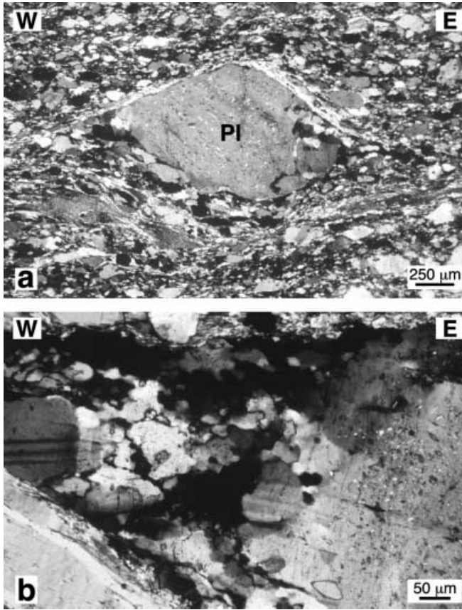
Fig. 14a, b DAV mylonites at Mühlbach (locality F, Fig. 1). a Plagioclase sigma-clast ( Pl ), showing crystal plastic deformation and incipient recrystallization, in a (sinistral) mylonitic orthogneiss. The foliation is defined by bands of extensively recrystallized quartz and feldspar. Foliation 177/70, lineation 081/02. b Enlargement from an adjacent sample, showing recrystallization of plagioclase by progressive subgrain rotation
