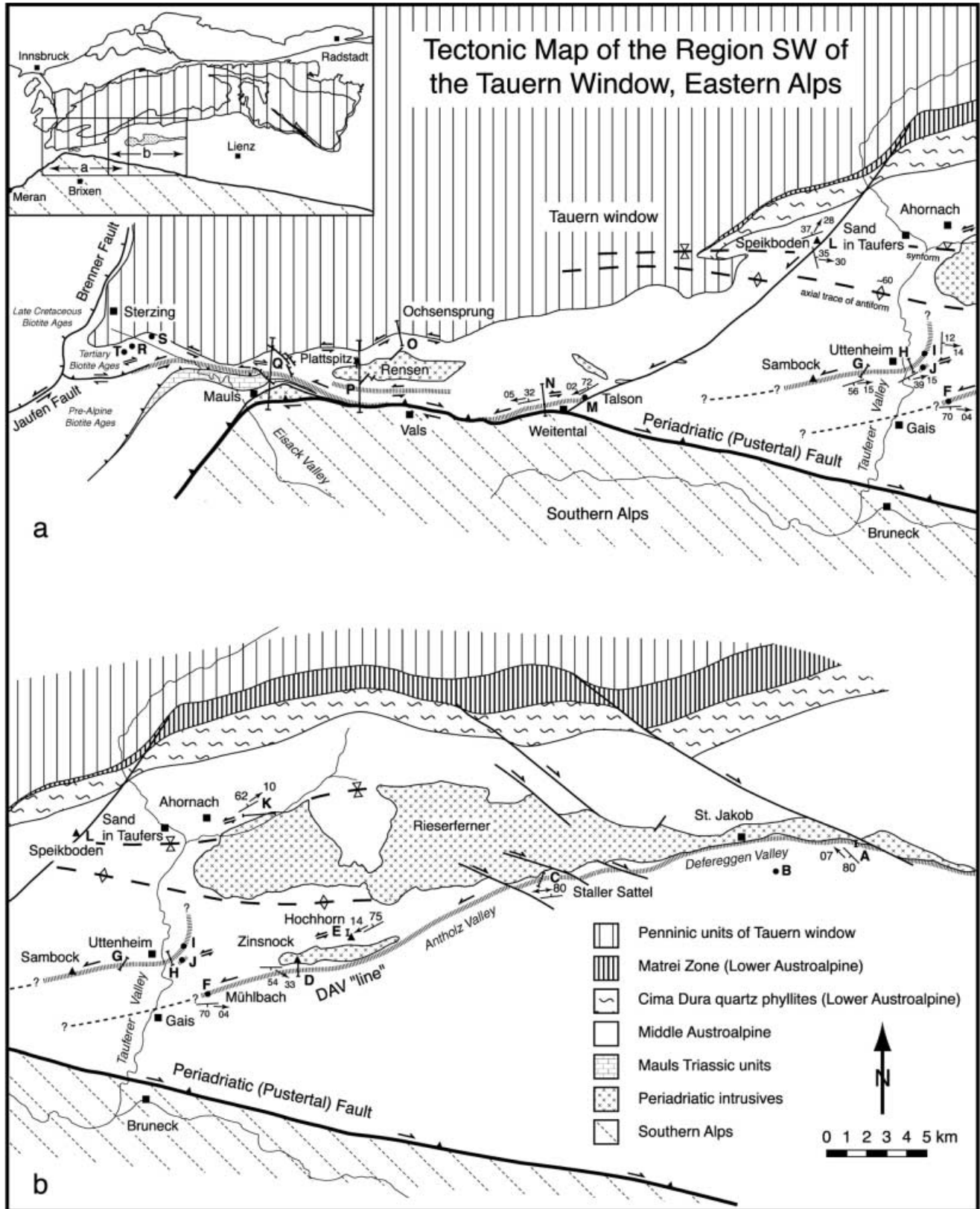
Fig. 1 Regional map of the Austroalpine south of the Tauern window, with locations referred to in the text indicated by bold letters . Note that the DAV "line" as indicated corresponds to the southern limit of heterogeneous Alpine sinistral overprint and is gradational to the north; the same applies to the dextral overprint in the western area around Maults-Sterzing, where
