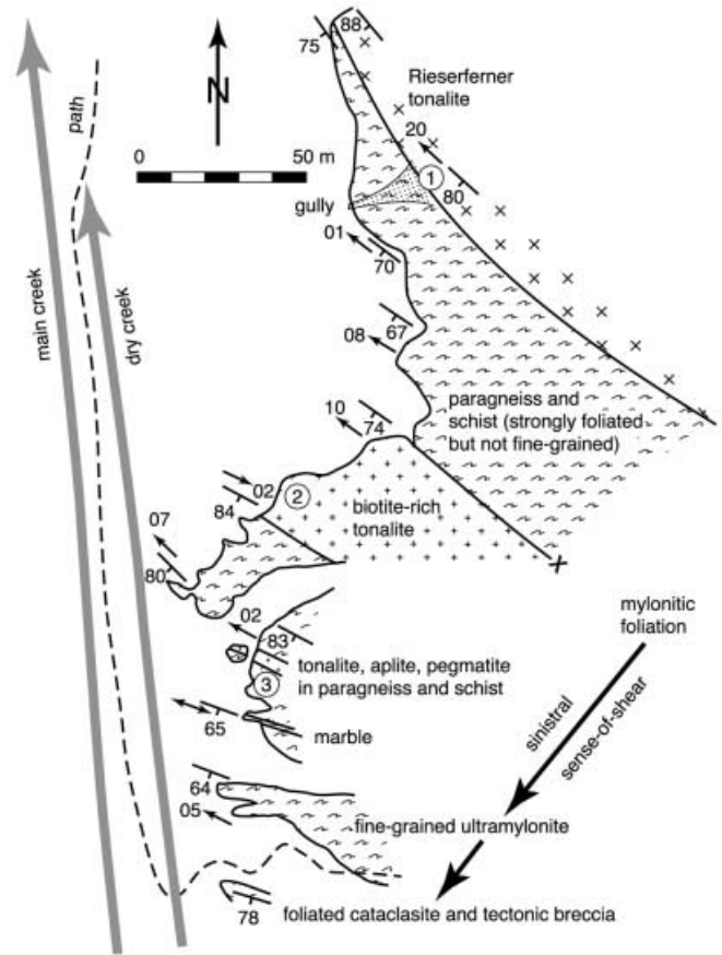
Fig. 9 Sketch map of the Stemmeringer Almbach locality (A in Fig. 1)
