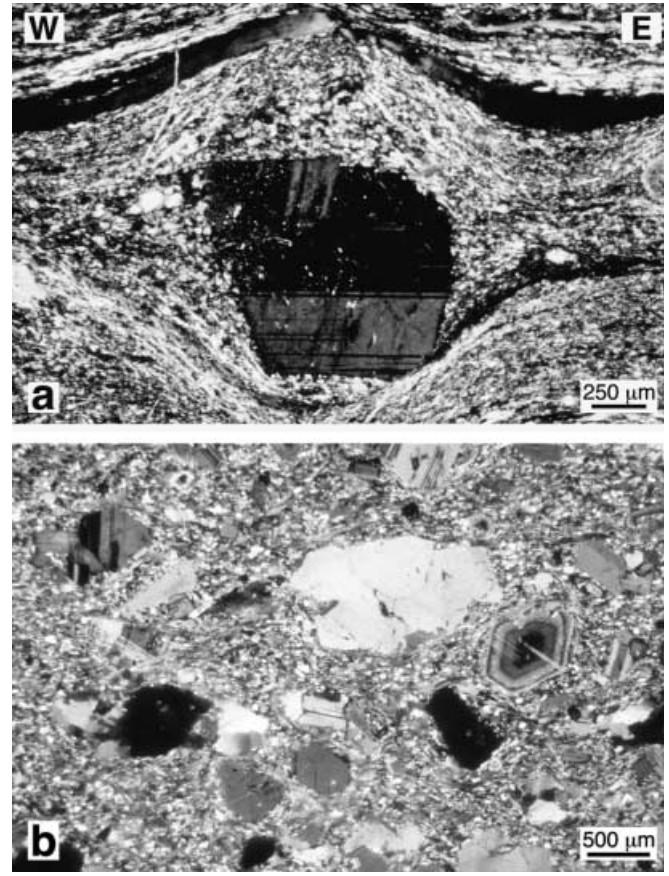
Fig. 17a, b Different microstructural aspect of Periadriatic dykes from the Plattspitz-Ochsenprung area. a Extreme (sinistral) mylonitization of the dated dyke BG169 ( 30.9 \pm 0.2 Ma; Müller et al. 2000), showing quartz ribbons wrapping around a plagioclase porphyroclast. The plagioclase acts mainly as a rigid clast, without significant crystal-plastic deformation, but does extensively recrystallize to a fine-grained matrix in the tails to either side. Foliation 355/56, lineation 079/07. b The opposite extreme, namely a practically undeformed “rhyodacitic” dyke similar to those dated by Kugel (1989) as ~30 Ma, i.e. only very
