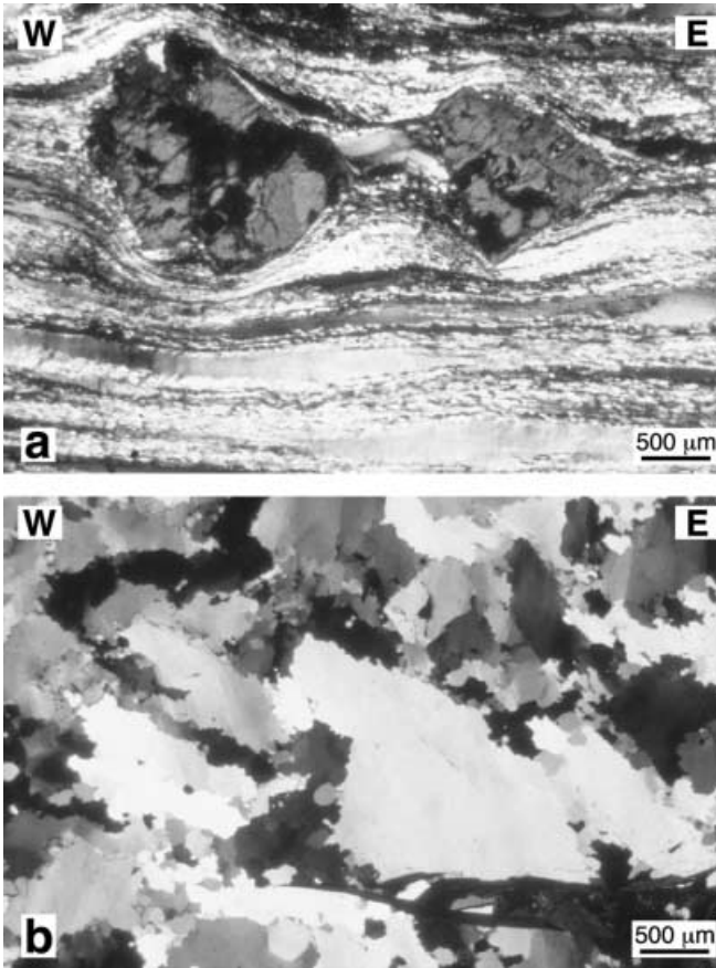
Fig. 16a, b Progressive change in quartz microstructure in the sinistral DAV mylonites from a south to b north. a Sample 1.5 km from the Tauern window contact, in the strongly mylonitic zone ~500 m south of the Rensen pluton. Bookshelf structure in fractured feldspar showing sinistral shear sense, with fine-grained recrystallization of quartz by progressive subgrain rotation. Foliation 336/53, lineation 251/04, from near point 2285 m, 1.3 km direction 170° from Plattspitz (BG69 from Grollmund 1996). b Sample ~50 m from the Tauern window contact at Ochsenprung, showing exaggerated grain growth of quartz by grain boundary migration. Shear sense still sinistral from oblique fabric and preferred orientation. Foliation 356/54, lineation 266/13 (BG101 from Grollmund 1996)
