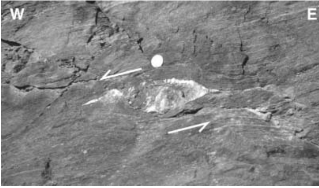
Fig. 18 Asymmetrical leucocratic boudin in prasinities (?Lower Austroalpine Matri Zone; see Fig. 1), indicating sinistral shear sense. Locality is at the contact to the Tauern window, on the road section near Valgnaun, north of Mault. View looking N, foliation 005/40, lineation 285/25
