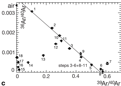
Fig. 8 a ^{40}\text{Ar} – ^{39}\text{Ar} stepwise-heating spectra, b corresponding mineral chemical discrimination diagram based on Ar isotopes and c isochron diagram for pseudotachylyte DAV97/16 from Speikboden (locality L). Sample locality is on the main ridge ~200 m ESE of the iron cross marking the Speikboden peak
