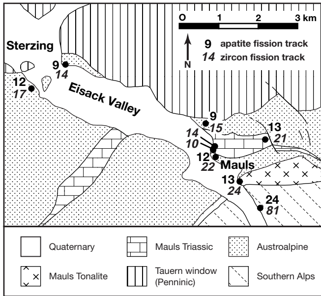
Fig. 2 Zircon ( italics ) and apatite ( roman ) fission-track ages in the SW Tauern window area, to either side of the Eisack valley south of Sterzing. Original data from Fügenschuh (1995) and Stöckli (1995)
