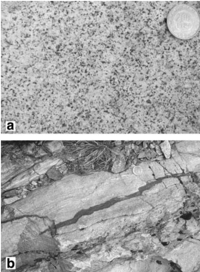
Fig. 12 a Undeformed Zinsnock tonalite that crosscuts the strongly foliated DAV mylonites in the adjacent contact aureole. In thin section, solid-state deformation is limited to undulose extinction and minor subgrain formation in quartz. b Pseudotachylyte generally concordant but locally crosscutting the DAV mylonitic foliation. Foliation 180/54, lineation 120/33. As noted in text, the lineation is typically steeper in the southernmost DAV mylonite exposures. The pseudotachylyte was sampled as DAV97/2 for Ar–Ar dating (see Fig. 13)
