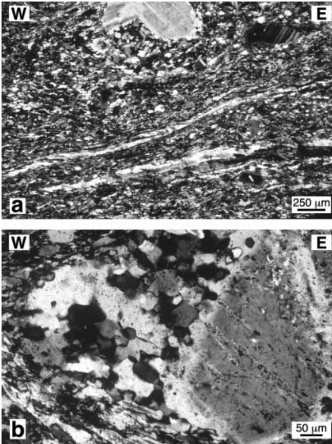
Fig. 20a, b Mylonitic fabric and plagioclase recrystallization in the Sprechenstein dyke. a Ribbon quartz development, with partial recrystallization by subgrain rotation, and plagioclase clast showing little evidence for crystal-plastic shape change but still partially recrystallized. b Close-up of plagioclase recrystallization by progressive subgrain rotation
