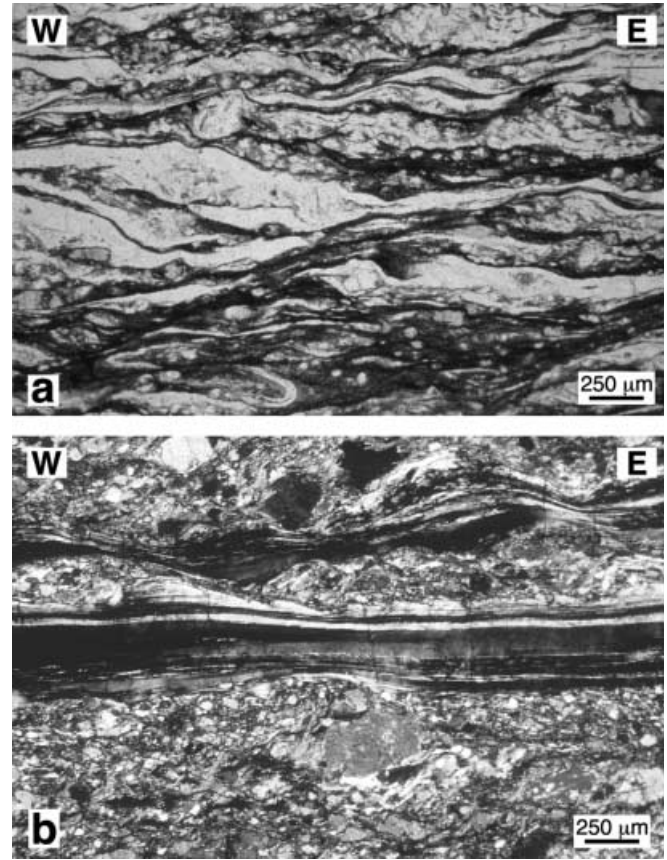
Fig. 21a, b Fabrics in the amphibolites from the dyke-bearing outcrops of a Reifenstein and b the Penserjoch road. a Sinistral mylonites with excellent shear bands in amphibole-bearing paragneiss immediately below the castle of Reifenstein (location R in Fig. 1). Ultrafine foliated brown layers with rounded clasts, both parallel to the foliation and to shear bands, could represent smeared-out pseudotachylytes. Approximately 50 m north of this outcrop, the more micaceous paragneisses and schists show common conjugate shear bands, but with sinistral sense dominant. Foliation 330/72, lineation 245/16. b Dextral mylonites from the northernmost part of the Penserjoch road outcrop (location T, Fig. 1). Note that the quartz recrystallization is very fine grained, similar to observations at the Sprechenstein location (Figs. 19, 20). However, continuous dextral shear bands in the adjacent amphibolite here show stable biotite and (fibrous) amphibole growth, so conditions at least initially were similar to those observed in the sinistral fabrics. Foliation 346/84, lineation 258/09
