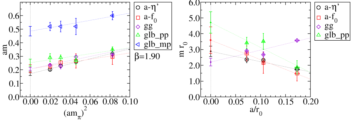
Figure 1: (Left) Mass spectrum (gg: gluino-gluon; glb_pp: glueball 0^{++} ; glb_mp: glueball 0^{-+} ) at \beta = 1.90 for four values of the a\pi mass. The extrapolated chiral limit is shown as well. (Right) Mass spectrum extrapolated to the continuum limit, using r_0 .
