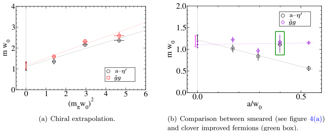
Figure 6. (a) Extrapolation of the a-\eta' and gluino-gluon ( \tilde{g}g ) masses to the chiral limit computed with tadpole improved clover fermions. (b) Comparison of the extrapolations to the continuum limit of the a-\eta' and gluino-gluon masses with the tadpole clover improved action results (green box).
