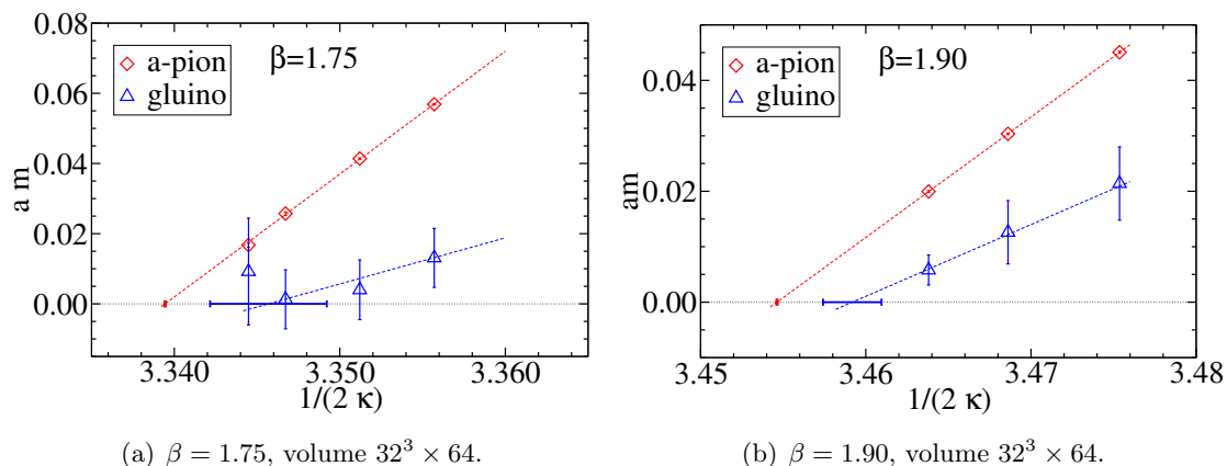
Figure 2. Comparison between the values of \kappa_c defined as the value of \kappa where the square of the a - \pi mass (a-pion) or the renormalised gluino mass am_S Z_S^{-1} (gluino) vanishes. The horizontal thick lines (red and blue) show the uncertainty in the determination of the intercept with zero.
