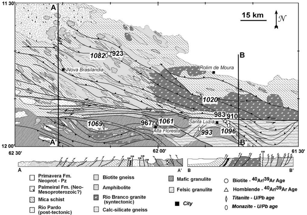
Figure 3. Map of portion of Nova Brasilândia belt compiled from regional maps (Rio Pardo and Paulo Saldanha 1:100,000 quadrangles by Bahia and Silva [1998] and Scandolaro and Rizzotto [1998]. Schematic cross sections indicate a regional structure with double vergence. Strike-slip mylonite zones with sinistral offset predominate in the central domain. Age data from U/Pb and ^{40}\text{Ar}/^{39}\text{Ar} analysis from this study are shown, indicating regional cooling after circa 1.05 Ga.
