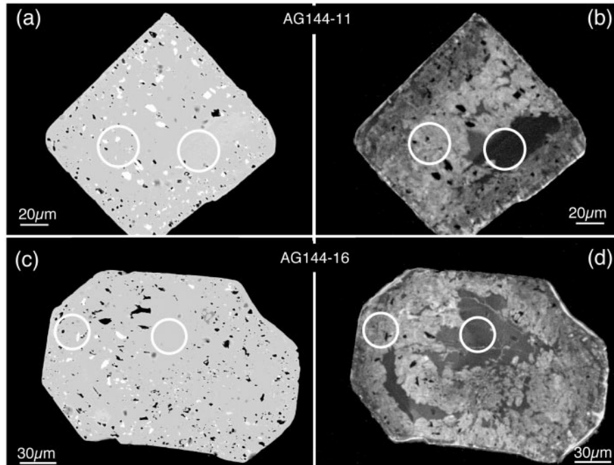
Fig. 5. Internal textures in BSE (left column) and CL images (right column) of zircons from the plagiogranitic fragment in the Grizzas breccia (AG144). Areas targeted with SHRIMP are circled, and codes correspond to results in Table 2. (a)–(d) Complex, partially altered zircons (type 2). Relict domains show low luminosity and are homogeneous in BSE image. Altered domains appear bright in CL image and are rich in inclusions. Dark spots in BSE image are voids of fluid inclusions; bright spots are Y–REE–Th-rich phases.
