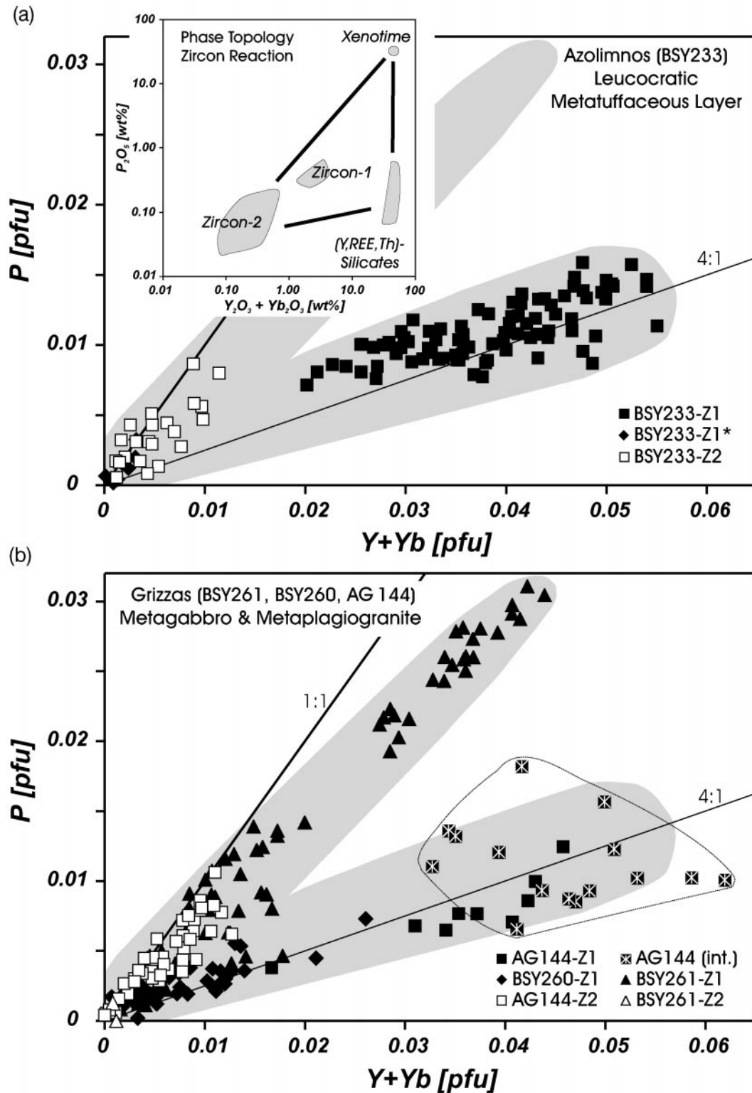
Fig. 8. Correlation between Y + Yb and P cations per zircon formula unit (see Table 1). Bold line indicates ideal xenotime substitution trend. Filled symbols denote analyses obtained on pristine (type 1) zircon; open symbols recrystallized domains and overgrowth rims. (a) Zircon analyses from the Azolimnos sample (Fig. 7); recrystallization decreases concentrations in trivalent cations and P. Inset graph represents the zircon reaction, including partial analyses of inclusion phases. (b) Zircons from the meta-igneous samples at Grizzas falling along the xenotime substitution and a P-poor trend. Grey-line envelope encloses reintegrated area scan analyses on porous, inclusion-rich zircon domains.
