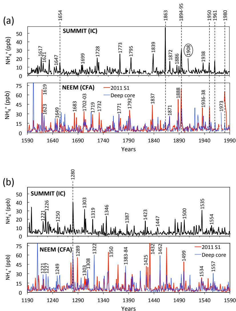
Figure 13. Comparison of ammonium records obtained at Summit and NEEM (NEEM-2011-S1 and the deep core) from 1590 to 1990 (a) and from 1190 to 1590 (b). All records are seasonally resolved, but data are presented here as annual means. Dashed lines denote the years for which a peak is identified in both cores. The Summit data are from Legrand and De Angelis (1996) and Savarino and Legrand (1998).
