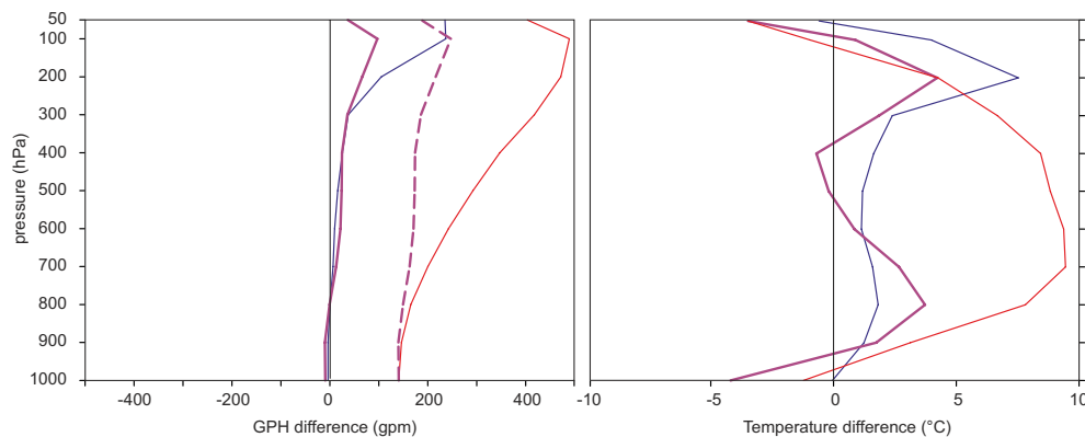
Fig. 5. Vertical profile of the difference between observations from the MS Schwabenland and 20CR for GPH (left) and temperature (right). Red = uncorrected profiles for the ascents #50–61, blue = all other ascents, thick purple = corrected profiles of ascents #50–61 (dashed: no altitude offset at 1000 hPa). Note that the 1000 hPa level was below sea level during ascents #50–61 and hence these values were extrapolated on the original data sheets.
