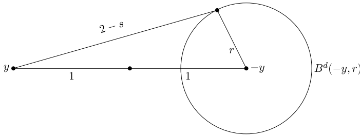
FIG. 1. Illustration of the argument used in the derivation of Theorem 7.17.
