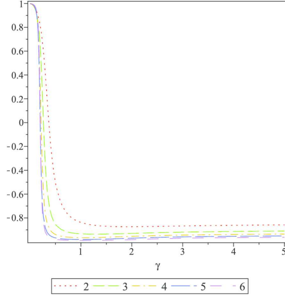
FIG. 2. \text{Cor}_{d-1,d}(\gamma) for d=2, \dots, 6 .
