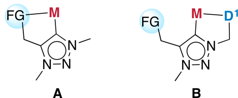
Figure 1 Functional group introduction in triazolylidenes induces either chelation ( A ) or provides an additional reactive group that can support the metal center ( B ).
