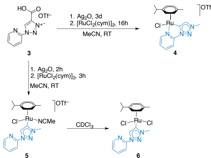
Scheme 2 Synthesis of complexes 4–6.
