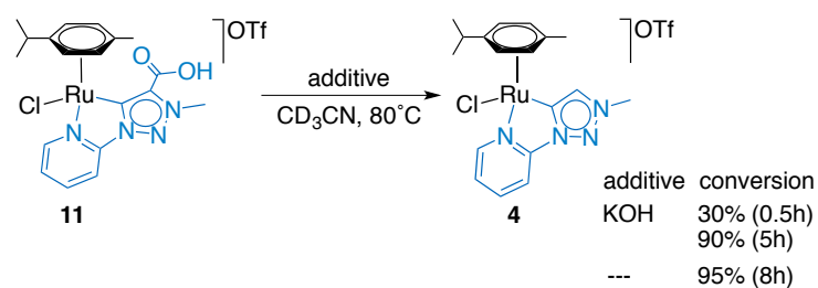
Scheme 6 Thermal and base-induced decarboxylation of complex 11 .
