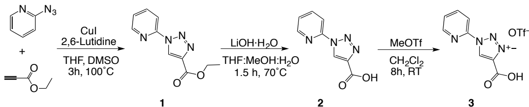
Scheme 1 Synthesis of triazolium salt 3 .
