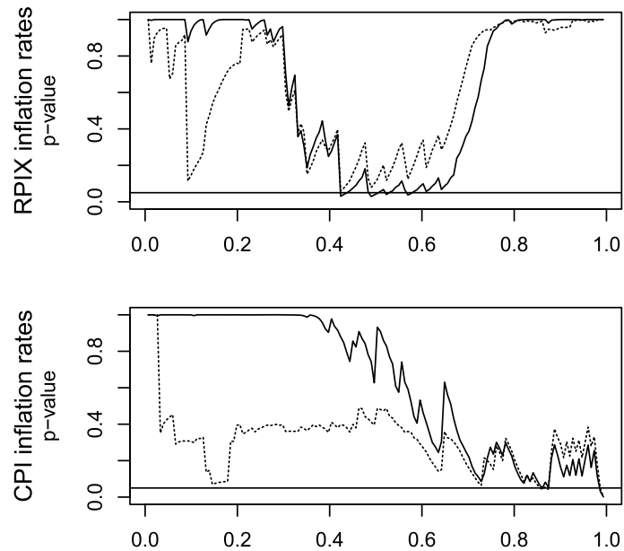
FIG 4. The p -values of the CEP tests for the AR forecast. The top panel corresponds to the prediction of RPIX inflation rates, whereas the bottom panel displays the results for CPI inflation rates. The solid horizontal lines give the 0.05 level; the solid lines refer to probabilistic calibration and the dotted lines refer to cross-calibration with respect to BoE.
