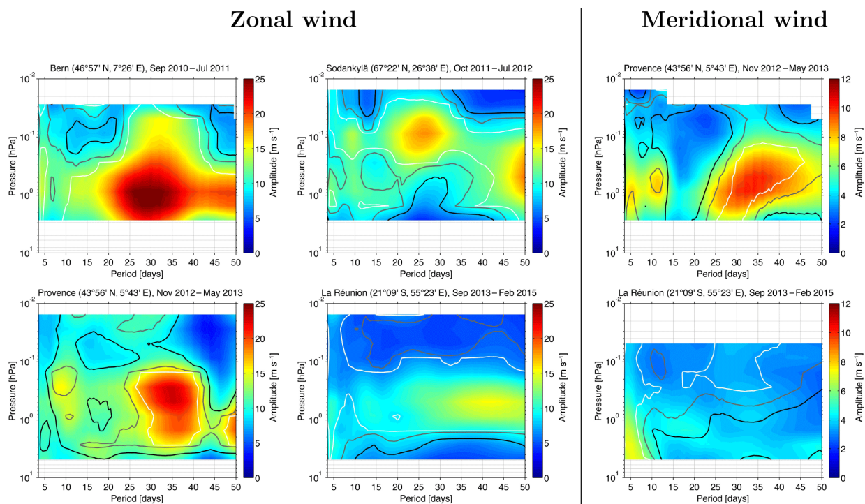
Figure 2. Temporally averaged periodograms of zonal and meridional wind profiles measured by WIRA. The black, gray and white contour lines mark \alpha = 0.5 , 0.1 and 0.01 , where the lowest value, i.e., the white contour, corresponds to the highest significance. The values of \alpha were calculated from Eqs. (5) and (6) based on the average oscillation amplitude and the noise of the entire wind measurement time series determined using the Allan standard deviation (detrended version of the standard deviation; e.g., Allan, 1966). The white areas represent altitudes and periods (i.e., window widths) for which the conditions of Eq. (4) are not satisfied, i.e., for which WIRA cannot provide reliable information due to an insufficient number of data points.
