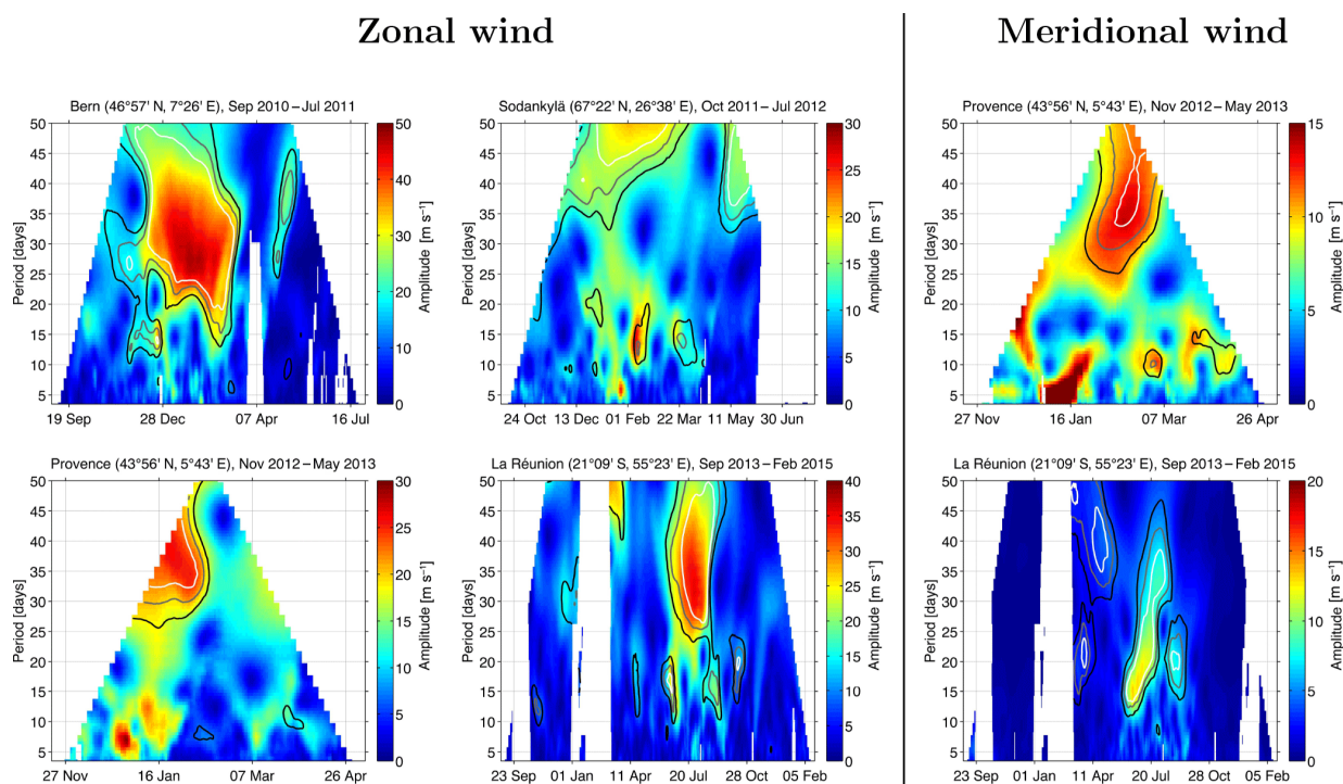
Figure 5. Temporal evolution of the periodogram at stratopause level (0.9 hPa) for wind measurements taken by WIRA. The black, gray and white contour lines mark \alpha = 0.5 , 0.1 and 0.01 according to Eq. (6). The lowest value, i.e., the white contour, corresponds to highest significance. White areas represent times for which \mathcal{B}_j contains indices before the start date or after the end date of the respective measurement campaign (which entails the trapezoidal shape of the colored area). Other areas are blanked out because the conditions of Eq. (4) are not satisfied, i.e., WIRA cannot provide reliable information due to an insufficient number of data points. Please note the occurrence of 16-day oscillations near the onset and the termination of the extra-long period oscillation in zonal wind for Bern and La Réunion.
