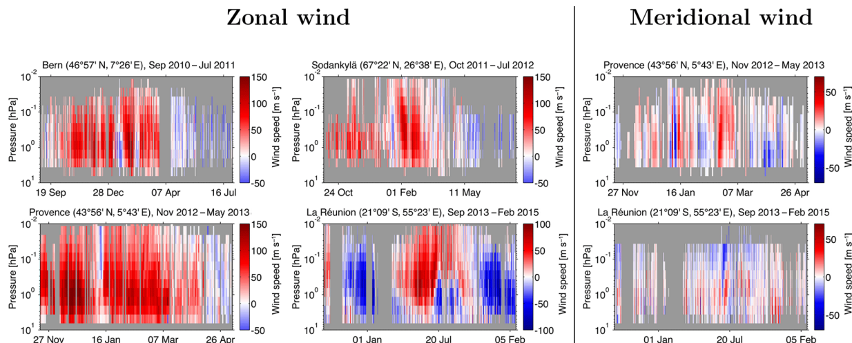
Figure 1. The zonal and meridional wind time series measured by WIRA during four different measurement campaigns analyzed in the present study. The gray areas correspond to data points judged untrustworthy according to the conditions indicated in the text. Please note the different color scale for zonal and meridional wind.
