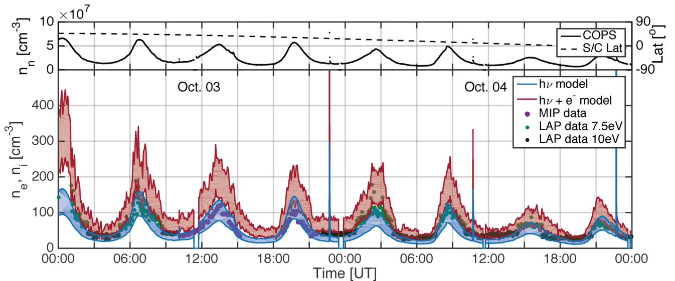
Figure 14. Top: ROSINA-COPS total neutral number density n_n(r_0) and the sub-spacecraft latitude as a function of time. Bottom: ionospheric density as a function of time. The period shown is 2014 October 03–04. The blue (red) curves correspond to the calculated ionospheric density assuming photoionization alone (photoionization and electron-impact ionization). The vertical spread of these curves corresponds to the range of ion outflow velocity considered, spreading from 400 \text{m s}^{-1} (top boundary) to 700 \text{m s}^{-1} (bottom boundary). The RPC-MIP electron density is shown with large, violet dots. There are no RPC-MIP data between 15:00 and 18:30 UT as the electron density was too low to be detected by the sensor in the LDL mode. The RPC-LAP electron density is shown with small green dots, assuming an electron temperature of 7.5 eV (light green for \xi \geq 7 \times 10^{19} \text{ cm}^{-1} ) or 10 eV (dark green for \xi < 7 \times 10^{19} \text{ cm}^{-1} ) (see Section 4.1).
