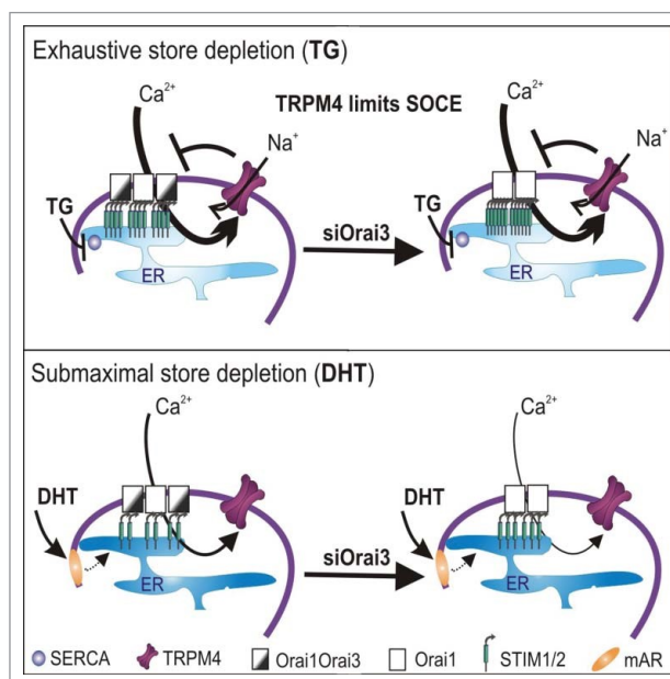
Figure 1. \text{Ca}^{2+} regulation in prostate cancer cells upon knockdown of Orai3. Upper panel: In prostate cancer cells, exhaustive store depletion by TG activates SOCE and subsequently TRPM4, as regulator of SOCE. An siRNA based knockdown of Orai3 does not reduce SOCE. Lower panel: Low SOCE signals do not activate TRPM4; thus, SOCE depends on the number of SOCE channels and the STIM/Orai ratio. siOrai3 reduces SOCE. Please see text for details.
