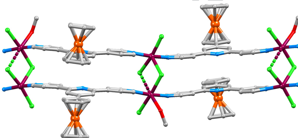
Fig. 1. Part of one double-stranded chain in the coordination polymer [\{\text{Cu}_2\text{Cl}_4(\mathbf{2})_2(\text{MeOH})\} \cdot 2.25\text{MeOH} \cdot \text{H}_2\text{O} \cdot \text{CHCl}_3]_n [6].
