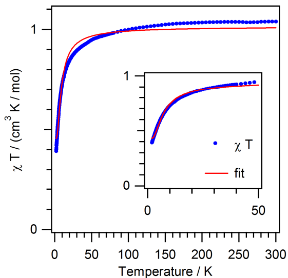
Fig. 6. Thermal variation of \chi_m T for 1 (per two Cu(II) ions); inset highlights the 50 to 1.9 K region. Solid lines represent fitted curves.
