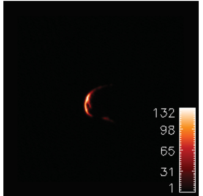
Figure 10. Phobos image, taken at 648.5 nm, as observed at 02:39:11 UT enhanced with a specific colourbar in order to better discern surface features. The colourbar values in the figure are in 10^{-5} \text{ W m}^{-2} \text{ sr}^{-1} \text{ nm}^{-1} .
