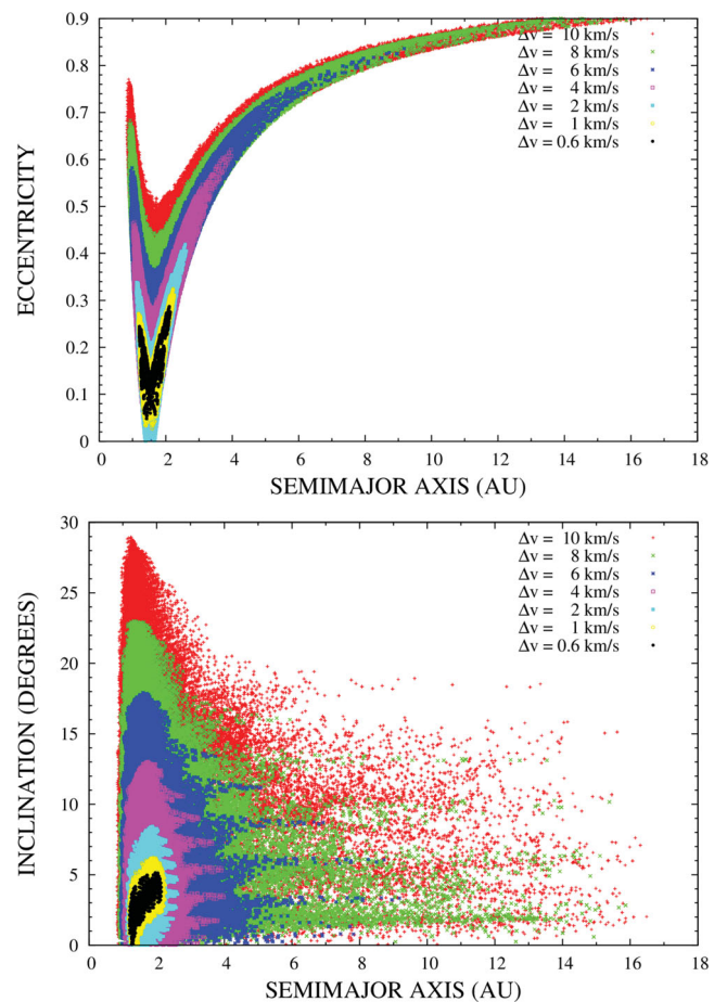
Figure 16. Same as Fig. 15 but for a primordial eccentricity of the captured Phobos of 0.8.
