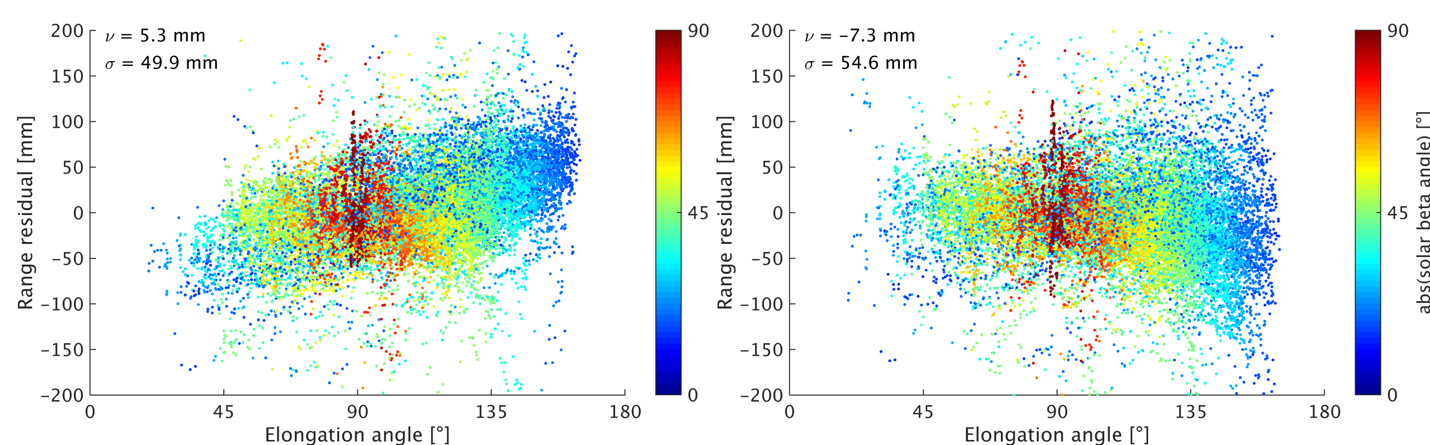
Figure 2: SLR residuals w.r.t. GLONASS-M orbits using the original ECOM (left) and the extended ECOM (right). Mean value ( \nu ) and standard deviation ( \sigma ) are based on all residuals whose absolute value is smaller than 150 mm. Observations to four GLONASS satellites (SVN 723, 725, 736, 737) have been excluded due to anomalous patterns. Furthermore, all residuals having an absolute beta angle smaller than 15^\circ have been not taken into account due to unmodeled attitude during eclipses.
