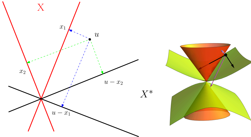
Figure 4: The bijection between critical points on X and critical points on X^* .
