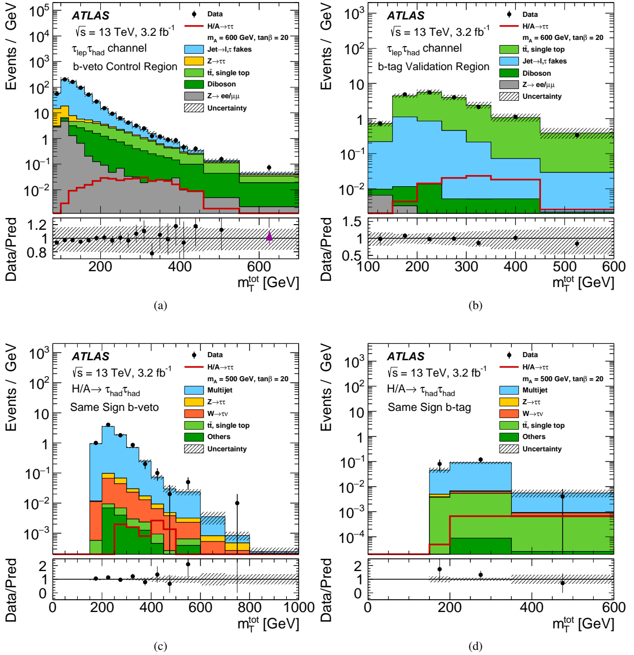
Figure 3: The distributions of m_T^{\text{tot}} in (a) the \tau_{\text{lep}}\tau_{\text{had}} channel W +jets control region, (b) the t\bar{t} validation region of the \tau_{\text{lep}}\tau_{\text{had}} channel, (c) the \tau_{\text{had}}\tau_{\text{had}} channel b -veto same-sign validation region and (d) the \tau_{\text{had}}\tau_{\text{had}} channel b -tag same-sign validation region. The various control and validation regions are defined in Table 1. The data are compared to the background prediction and a hypothetical MSSM H/A \rightarrow \tau\tau signal ( m_A = 500\text{GeV} and \tan\beta = 20 ). The Monte Carlo statistics of the signal is limited in the background-dominated regions. The label “Others” in (c) and (d) refers to contributions due to diboson, Z(\rightarrow \ell\ell) +jets and W(\rightarrow \ell\nu) +jets production. The background uncertainty includes statistical and systematic uncertainties. The bins have a varying size and overflows are included in the last bin of the distributions.
