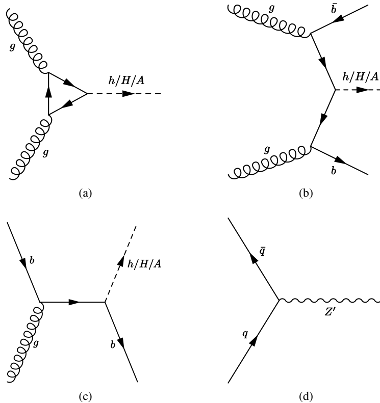
Figure 1: Lowest-order Feynman diagrams for (a) gluon–gluon fusion and b -associated production in the (b) four-flavour and (c) five-flavour schemes of a neutral MSSM Higgs boson. Feynman diagram for Drell–Yan production of a Z' boson at lowest order (d).
