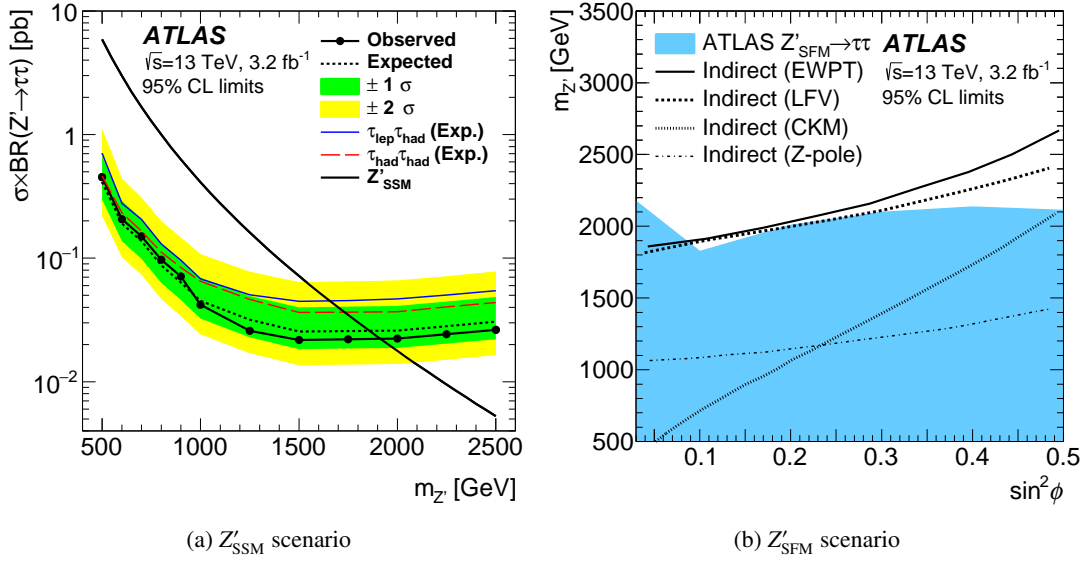
Figure 6: The 95% CL upper limit on the cross section times branching fraction for a Z' \rightarrow \tau\tau in (a) the Sequential Standard Model and 95% CL exclusion on (b) the SFM parameter space, overlaid with indirect limits at 95% CL from fits to electroweak precision measurements [131], lepton flavour violation [132], CKM unitarity [133] and Z-pole measurements [41].
