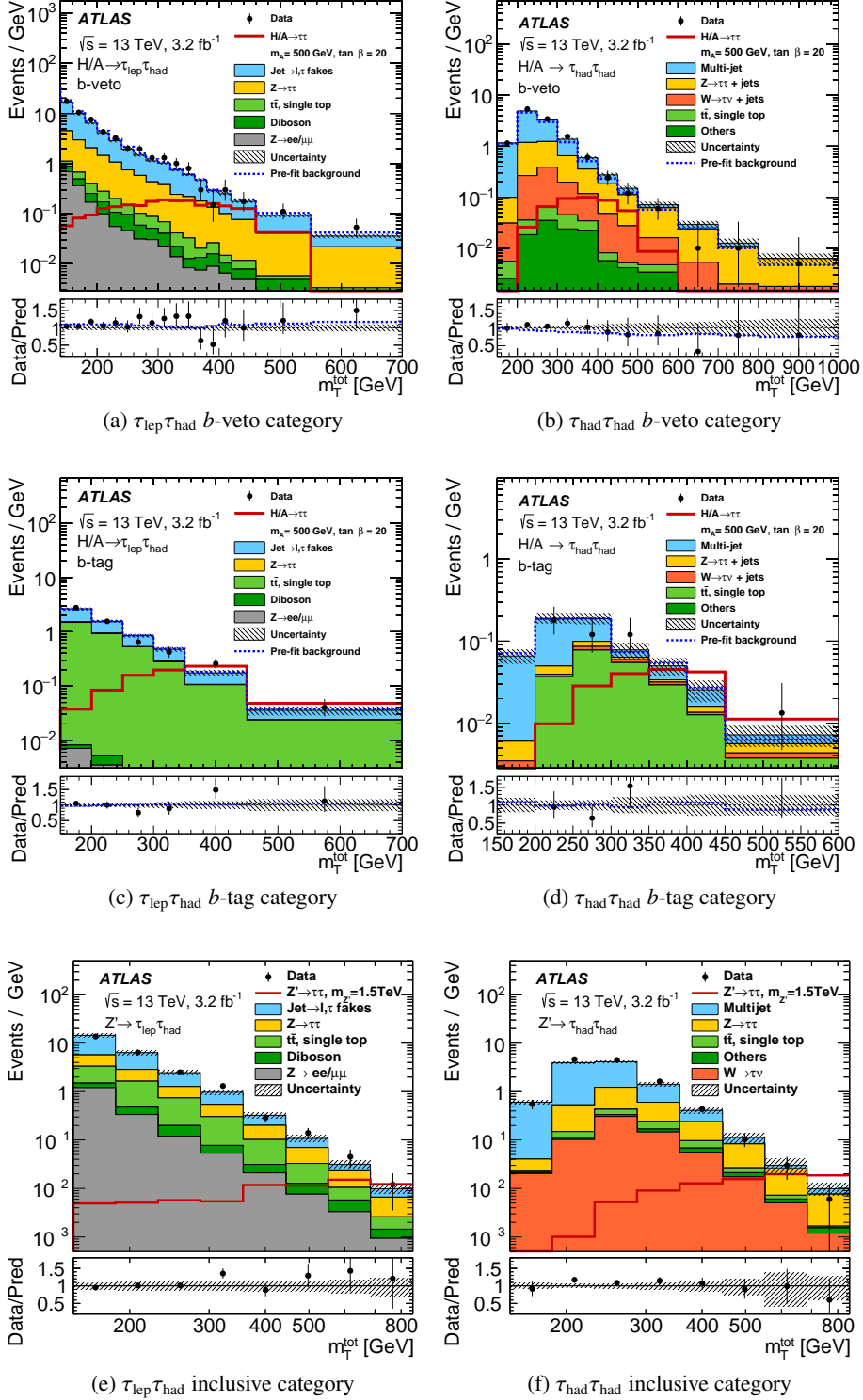
Figure 4: The distribution of m_T^{\text{tot}} for the b -veto category of the (a) \tau_{\text{lep}}\tau_{\text{had}} and (b) \tau_{\text{had}}\tau_{\text{had}} channels, the b -tag category of the (c) \tau_{\text{lep}}\tau_{\text{had}} and (d) \tau_{\text{had}}\tau_{\text{had}} channels, and the inclusive category of the (e) \tau_{\text{lep}}\tau_{\text{had}} and (f) \tau_{\text{had}}\tau_{\text{had}} channels. The label “Others” in (b), (d) and (f) refers to contributions due to diboson, Z(\rightarrow \ell\ell)+\text{jets} and W(\rightarrow \ell\nu)+\text{jets} production. For the b -veto and b -tag categories, the binning displayed is that entering into the statistical fit discussed in Section 7, while the predictions and uncertainties for the background and signal processes are obtained from the fit under the hypothesis of no signal. The inclusive category distributions are shown before any statistical fit. Overflows are included in the last bin of the distributions.
