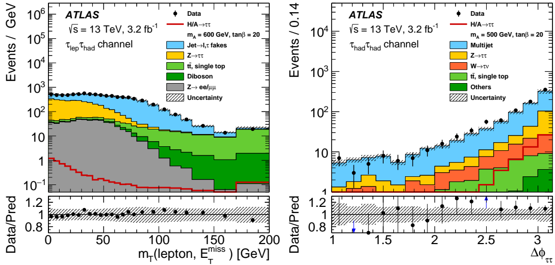
Figure 2: The distributions of (a) m_{\text{T}}(\ell, E_{\text{T}}^{\text{miss}}) in the \tau_{\text{lep}}\tau_{\text{had}} channel and (b) \Delta\phi(\tau_{\text{had-vis},1}, \tau_{\text{had-vis},2}) for the \tau_{\text{had}}\tau_{\text{had}} channel for the inclusive selection with the criterion for the variable displayed removed. The label “Others” in (b) refers to contributions due to diboson, Z(\rightarrow \ell\ell)+\text{jets} and W(\rightarrow \ell\nu)+\text{jets} production. Bins have a varying size and overflows are included in the last bin of the distribution on the left.
