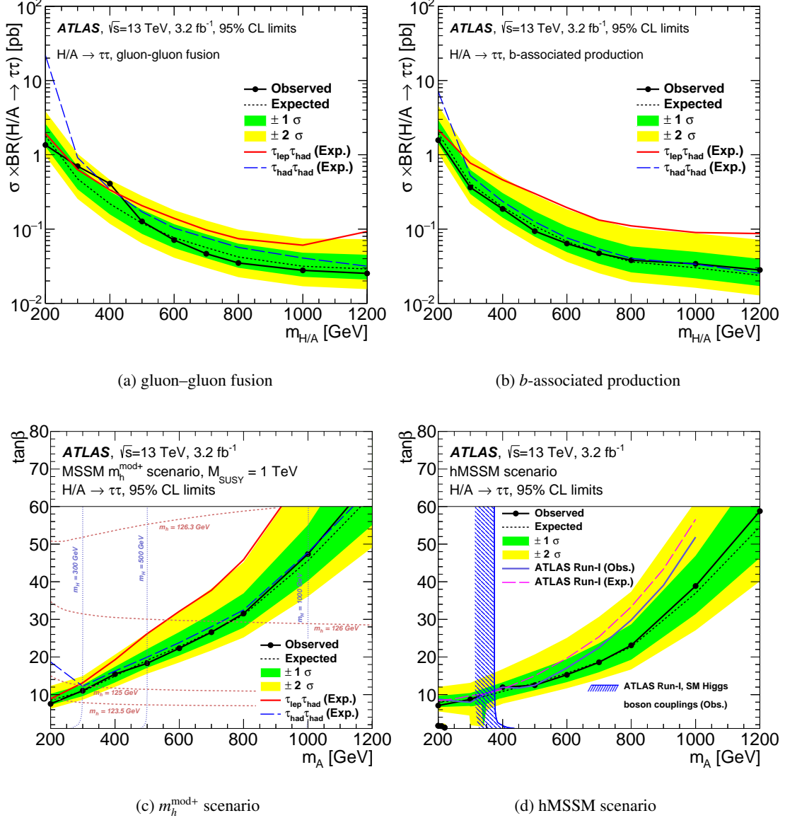
Figure 5: The observed and expected 95% CL upper limits on the production cross section times branching fraction of a scalar particle are shown for the combination of the \tau_{\text{lep}}\tau_{\text{had}} and the \tau_{\text{had}}\tau_{\text{had}} channels. The production mechanism of H/A \rightarrow \tau\tau is assumed to be (a) gluon-gluon fusion or (b) b -associated production. For comparison, the expected limits for the individual channels, \tau_{\text{lep}}\tau_{\text{had}} and \tau_{\text{had}}\tau_{\text{had}} , are shown as well. The observed and expected 95% CL limits on \tan\beta as a function of m_A are shown in (c) for the MSSM m_h^{\text{mod}+} scenario and (d) for the hMSSM scenario. For comparison, the expected limits from the individual channels, \tau_{\text{lep}}\tau_{\text{had}} and \tau_{\text{had}}\tau_{\text{had}} , are given in (c), while the observed and expected limits from the ATLAS Run-1 analysis in Ref. [28] are shown in (d). Dashed lines of constant m_h and m_H are shown in red and blue, respectively.
