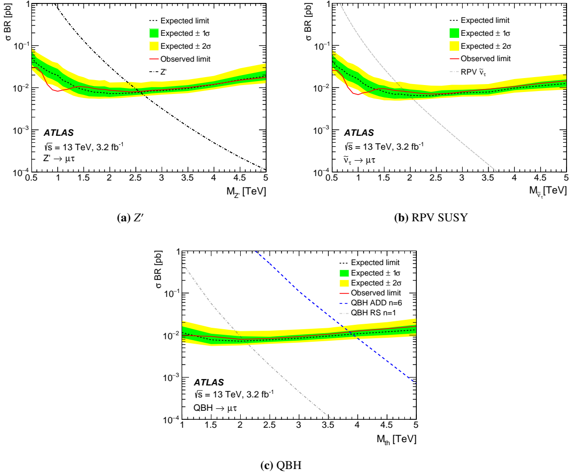
Figure 4: The observed and expected 95% credibility level upper limits on the (a) Z' , (b) \tau sneutrino ( \tilde{\nu}_\tau ) and (c) QBH ADD and RS production cross-section times branching ratio in decays to an \mu\tau final state. The signal theoretical cross-section times branching ratio lines for the Z' model, the QBH ADD model assuming six extra dimensions and the RS model with one extra dimension are obtained from the Monte Carlo generators simulating each process, while the RPV SUSY \tilde{\nu}_\tau includes the NLO K -factor calculated using LoopTools [37]. The expected limits are plotted with the \pm 1 and \pm 2 standard deviation uncertainty bands.
