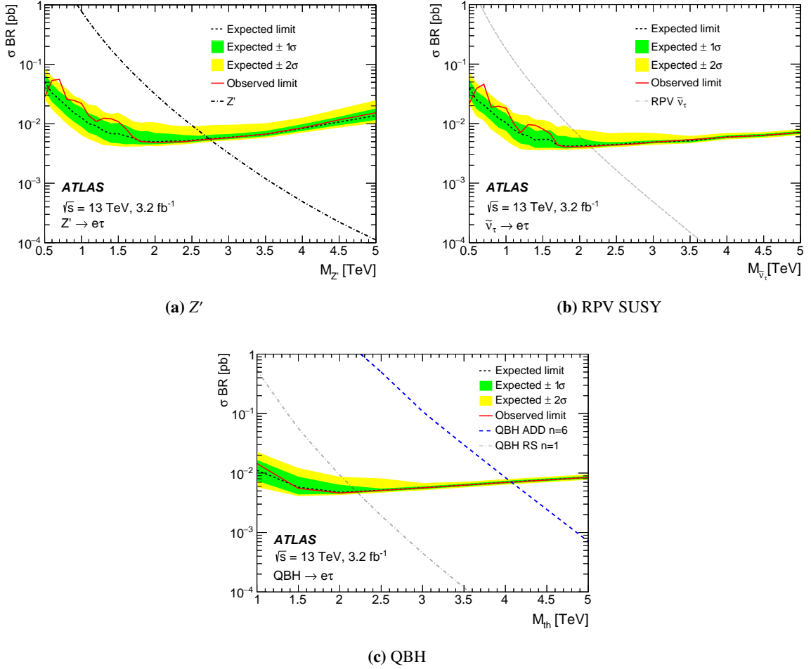
Figure 3: The observed and expected 95% credibility level upper limits on the (a) Z' , (b) \tau sneutrino ( \tilde{\nu}_\tau ) and (c) QBH ADD and RS production cross-section times branching ratio in decays to an e\tau final state. The signal theoretical cross-section times branching ratio lines for the Z' model, the QBH ADD model assuming six extra dimensions and the RS model with one extra dimension are obtained from the Monte Carlo generators simulating each process, while the RPV SUSY \tilde{\nu}_\tau includes the NLO K -factor calculated using LoopTools [37]. The expected limits are plotted with the \pm 1 and \pm 2 standard deviation uncertainty bands.
