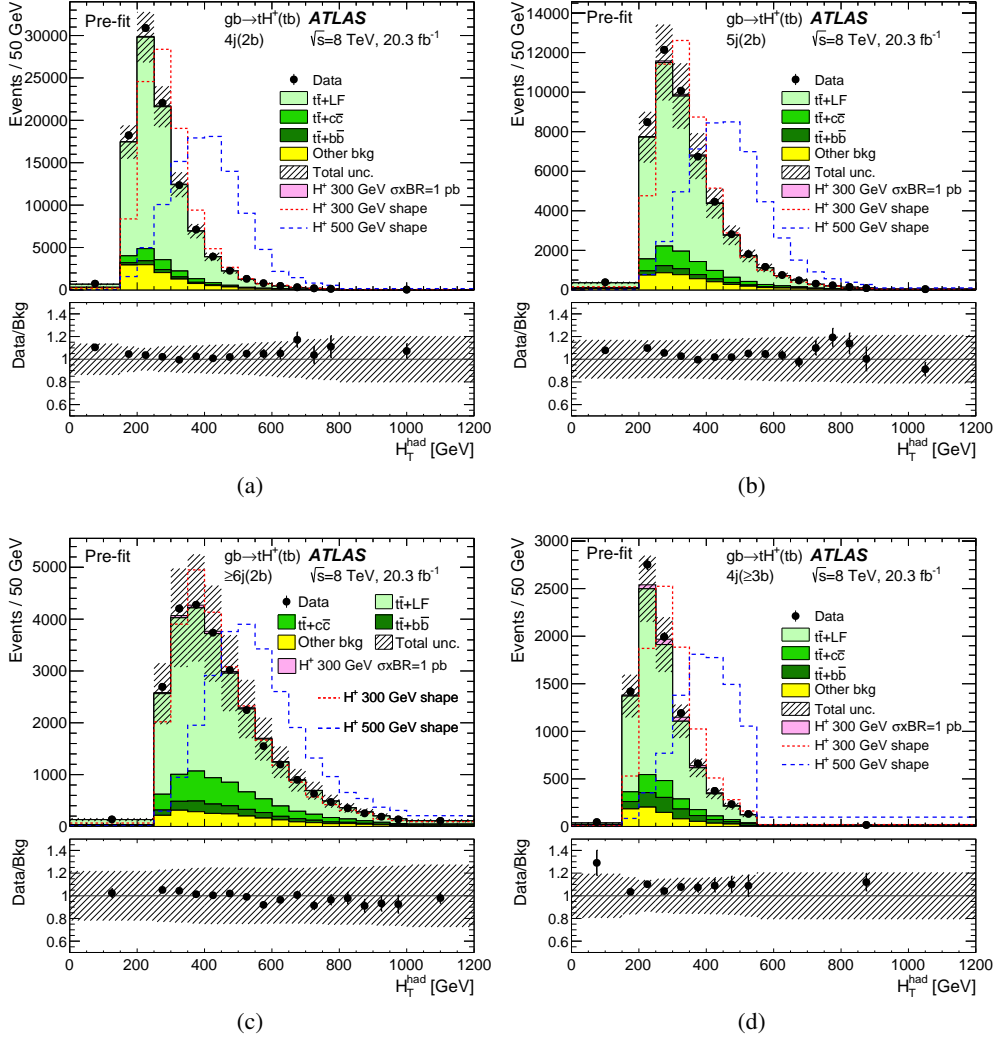
Figure 2: Pre-fit distributions of the scalar sum of the p_T of all selected jets, H_T^{\text{had}} , for the four control regions: (a) 4j(2b), (b) 5j(2b), (c) \geq 6j(2b) , (d) 4j( \geq 3b ). Each background process is normalised according to its cross section. A signal with m_{H^+} = 300 GeV, normalised to a production cross section times branching fraction for H^+ \rightarrow tb ( \sigma \times \text{BR} ) of 1 pb, is shown in pink, stacked on top of the background. Two signal shapes are shown superimposed as dashed lines normalised to the data. The last bin includes the overflow. The hatched bands show the pre-fit uncertainties, which are dominated by systematic uncertainties (discussed in section 4.3). The lower panels display the ratio of the data to the total predicted background.
